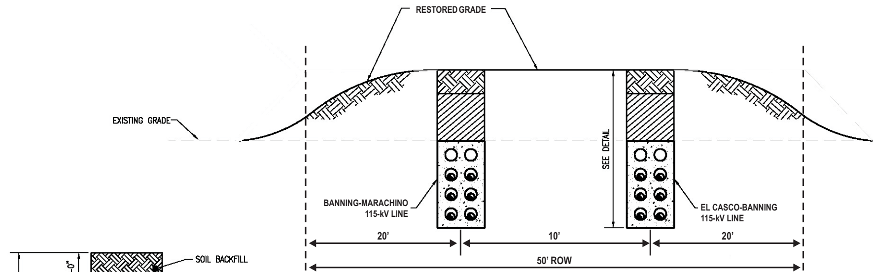
PROFILE VIEW - LOOKING EAST 115kV DUCTBANK CONSTRUCTION
