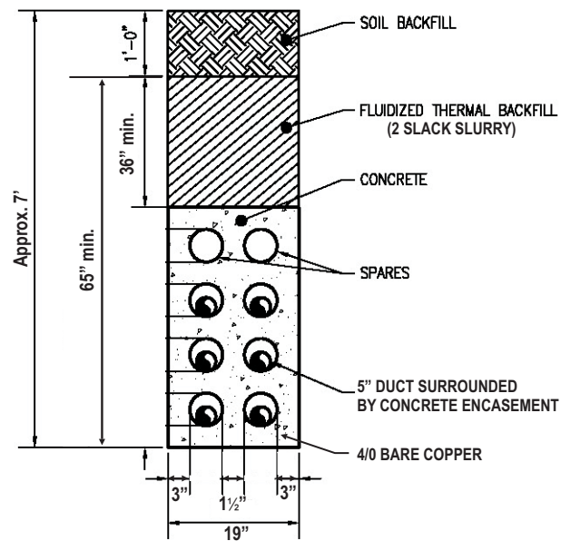
DETAIL 115kV DUCTBANK CONSTRUCTION
