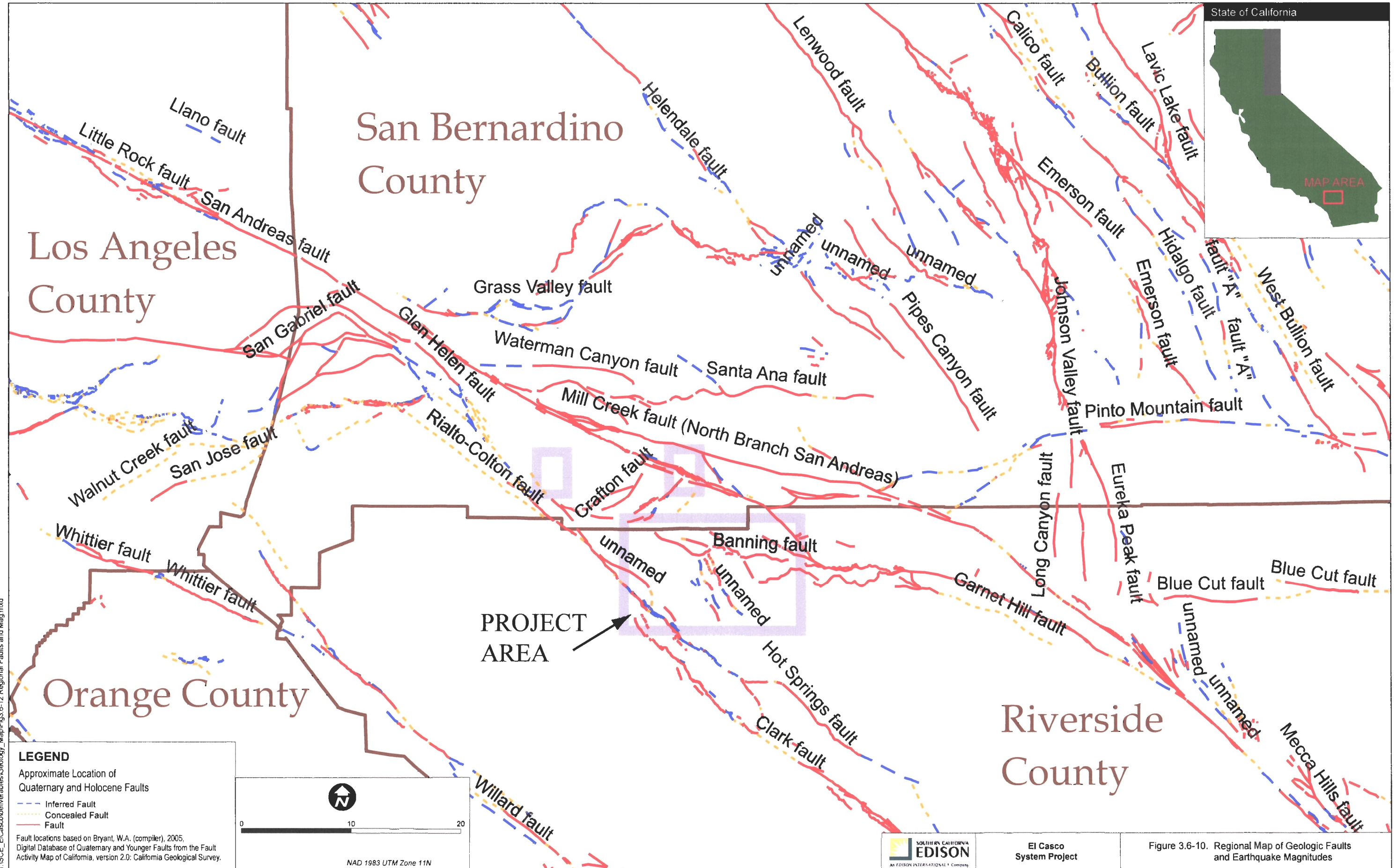
Figure 3.6-10, Regional Map of Geologic Faults
