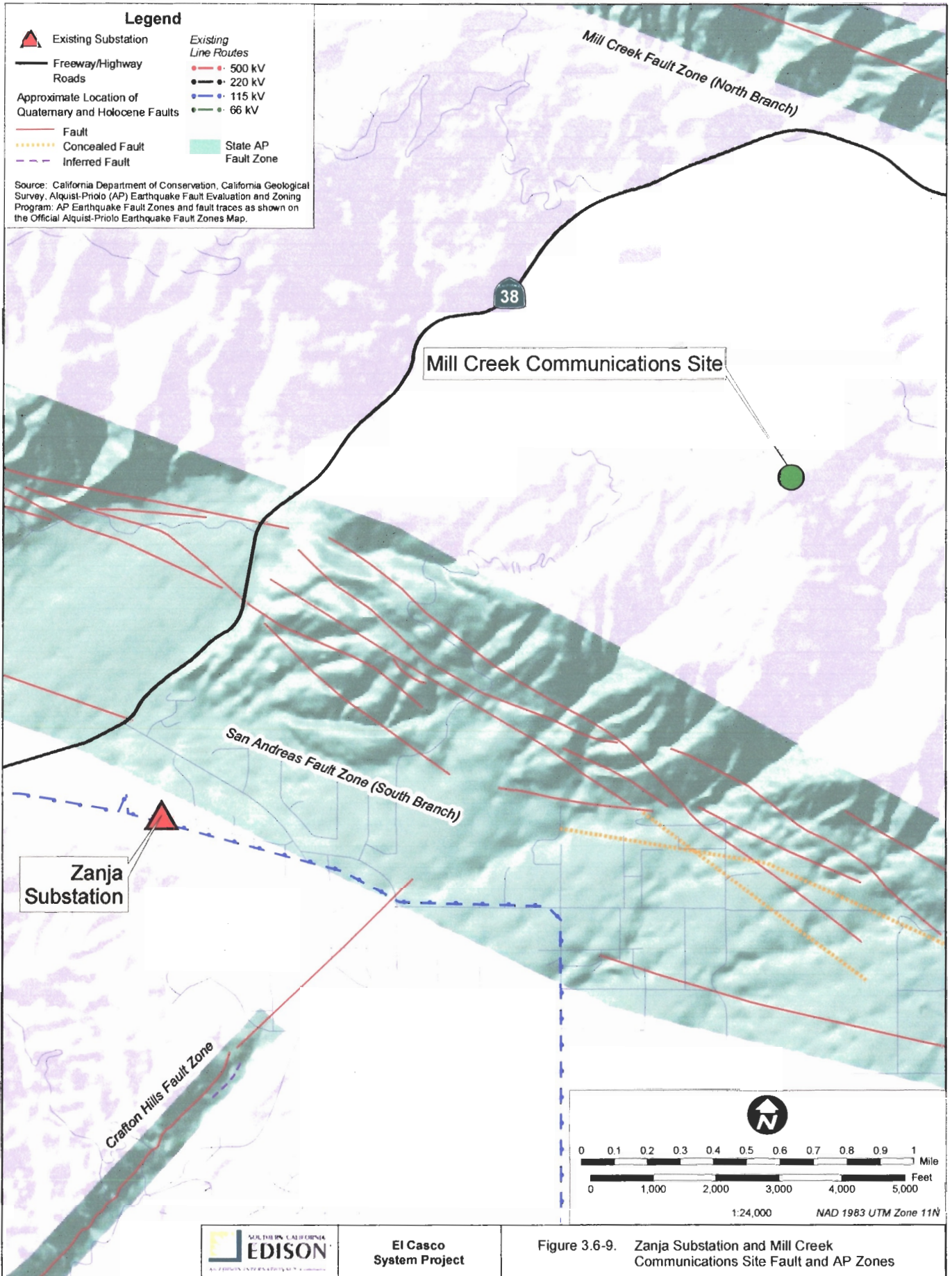
Figure 3.6-9, Zanja Substation and Mill Creek Communications Site Faults and AP Zones
