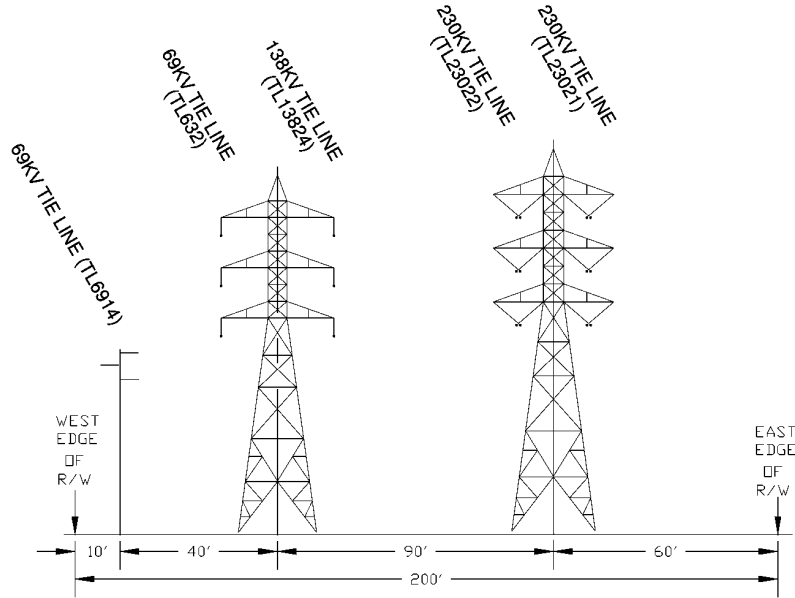
Existing Alignment
