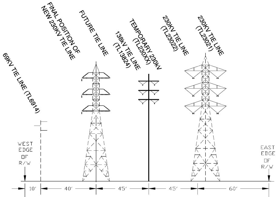
Temporary Alignment
