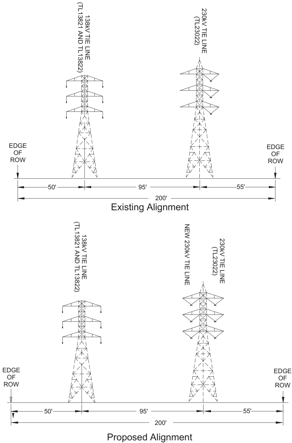
San Diego Gas and Electric Miguel–Mission 230kV #2 Project Figure 1-6: Existing and Proposed Cross-section of Subsection F
