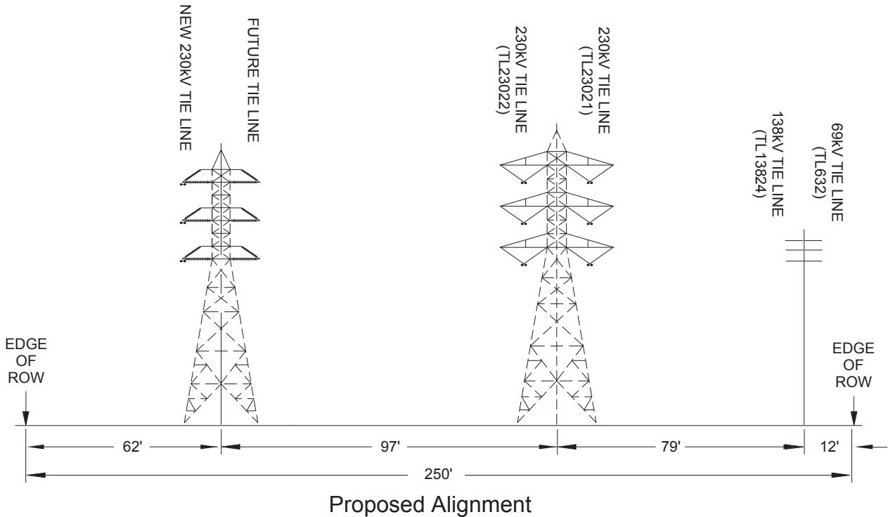
San Diego Gas and Electric Miguel-Mission 230kV #2 Project Figure 1-7c: Existing and Proposed Cross-section of Subsection A (Twr #40 - Twr #28)
