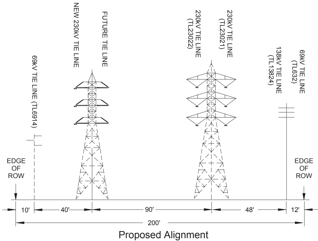
San Diego Gas and Electric Miguel-Mission 230kV #2 Project Figure 1-8a: Existing and Proposed Cross-section of Subsection B (Twr #28 - Twr #12)
