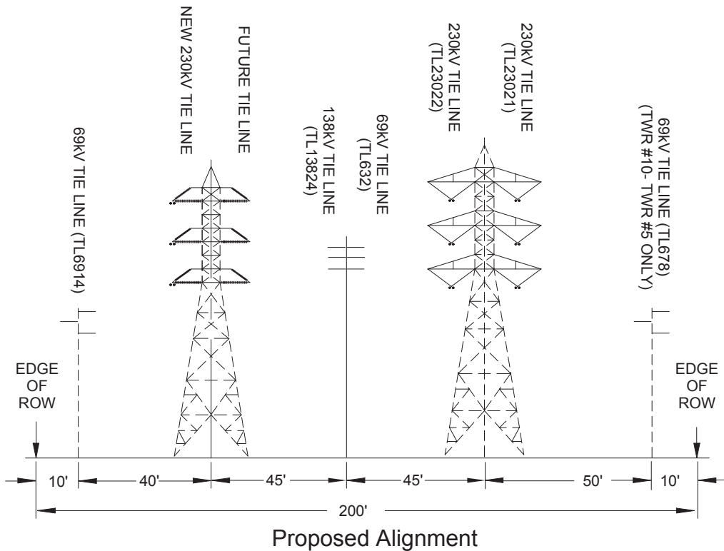
San Diego Gas and Electric Miguel-Mission 230kV #2 Project Figure 1-8b: Existing and Proposed Cross-section of Subsection B (Twr #12 - Twr #5)
