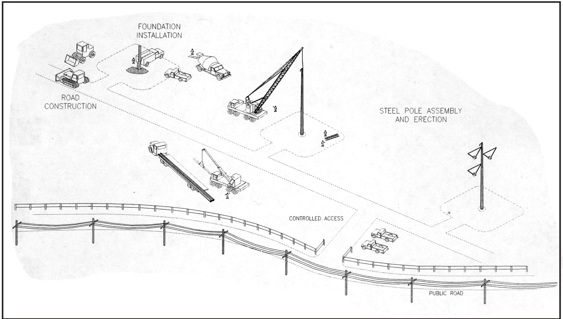
San Diego Gas and Electric Miguel Mission 230kV #2 Project Figure 1-12: Typical Transition Construction Activities
