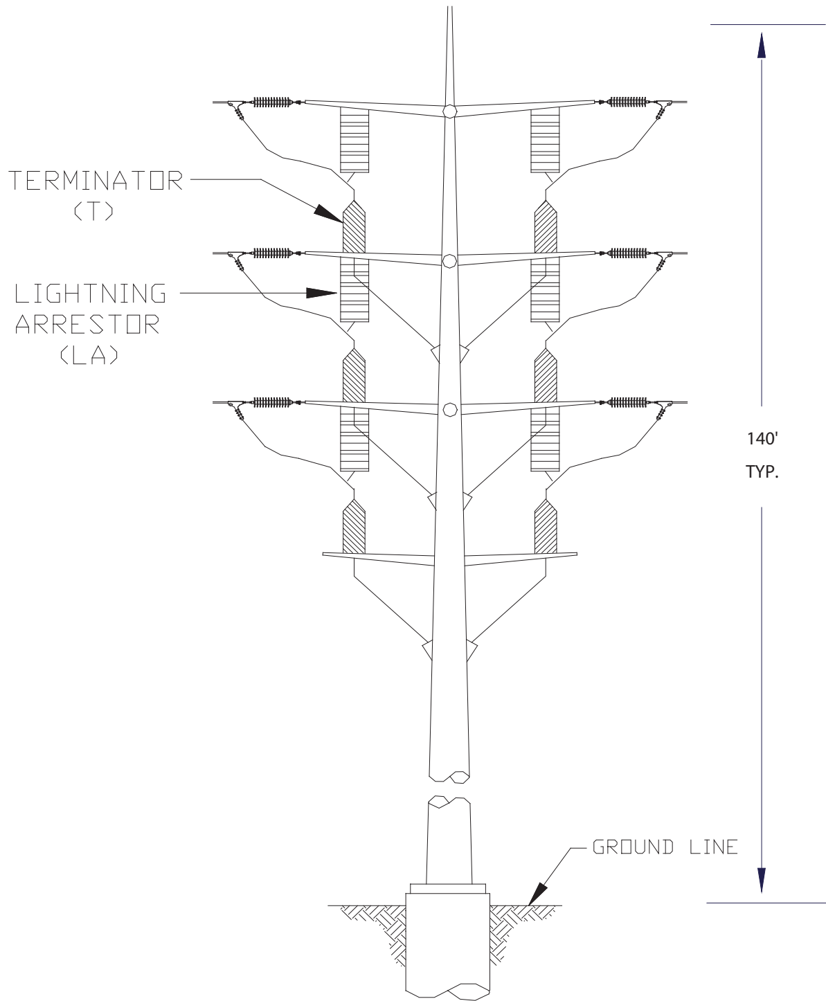
230kV CABLE POLE ELEVATION
