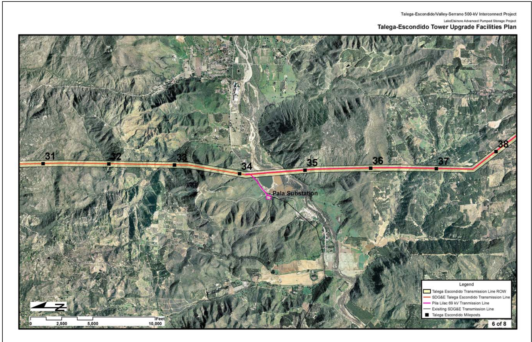
Figure 3.6.3-2: Talega-Escondido 230 kV Line Upgrade Map (6 of 8)
