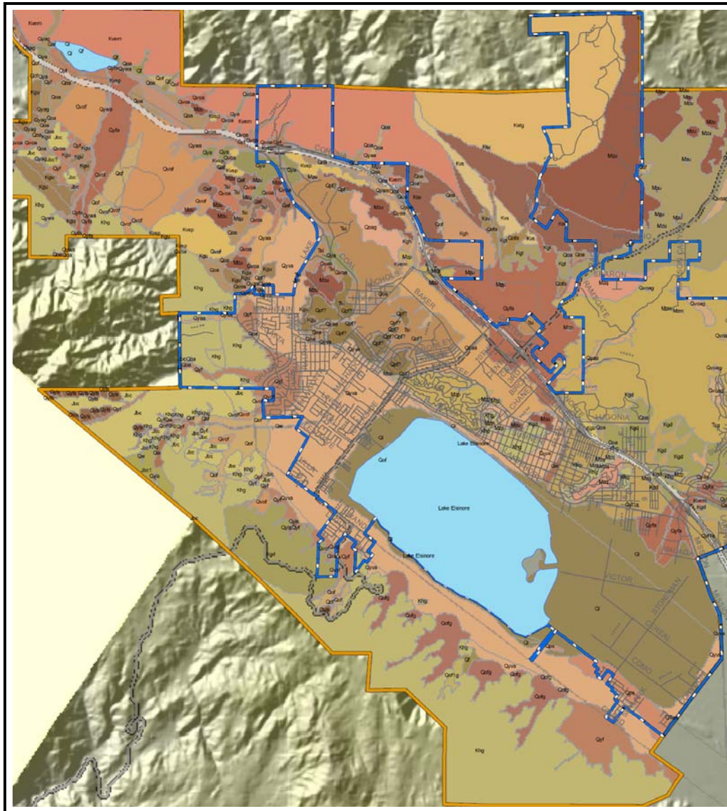
Figure 4.8.1-2. City of Lake Elsinore Geologic Formations Source: City of Lake Elsinore
