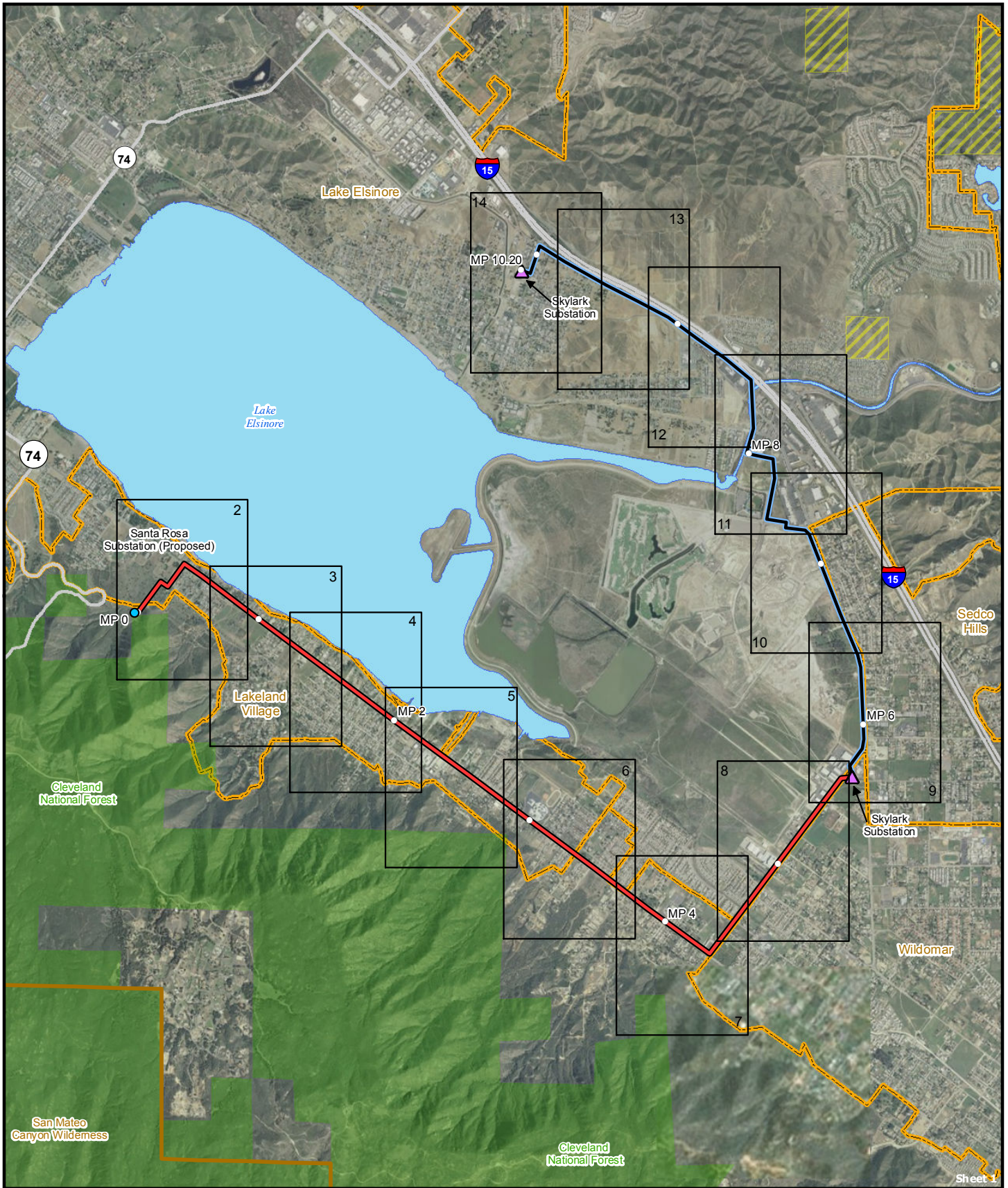
DRAFT 3/11 Figure Ap. 1b-1 Proposed 115 kV Route
