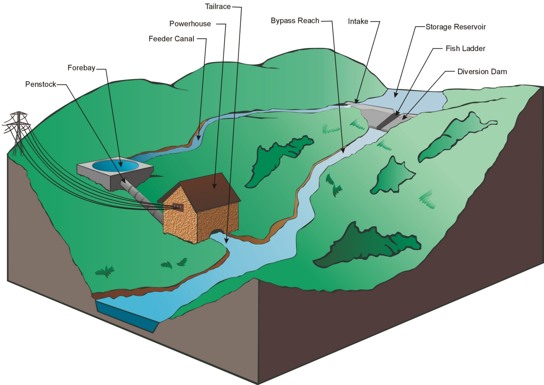
Figure 2 Typical Features of a Hydroelectric Plant
