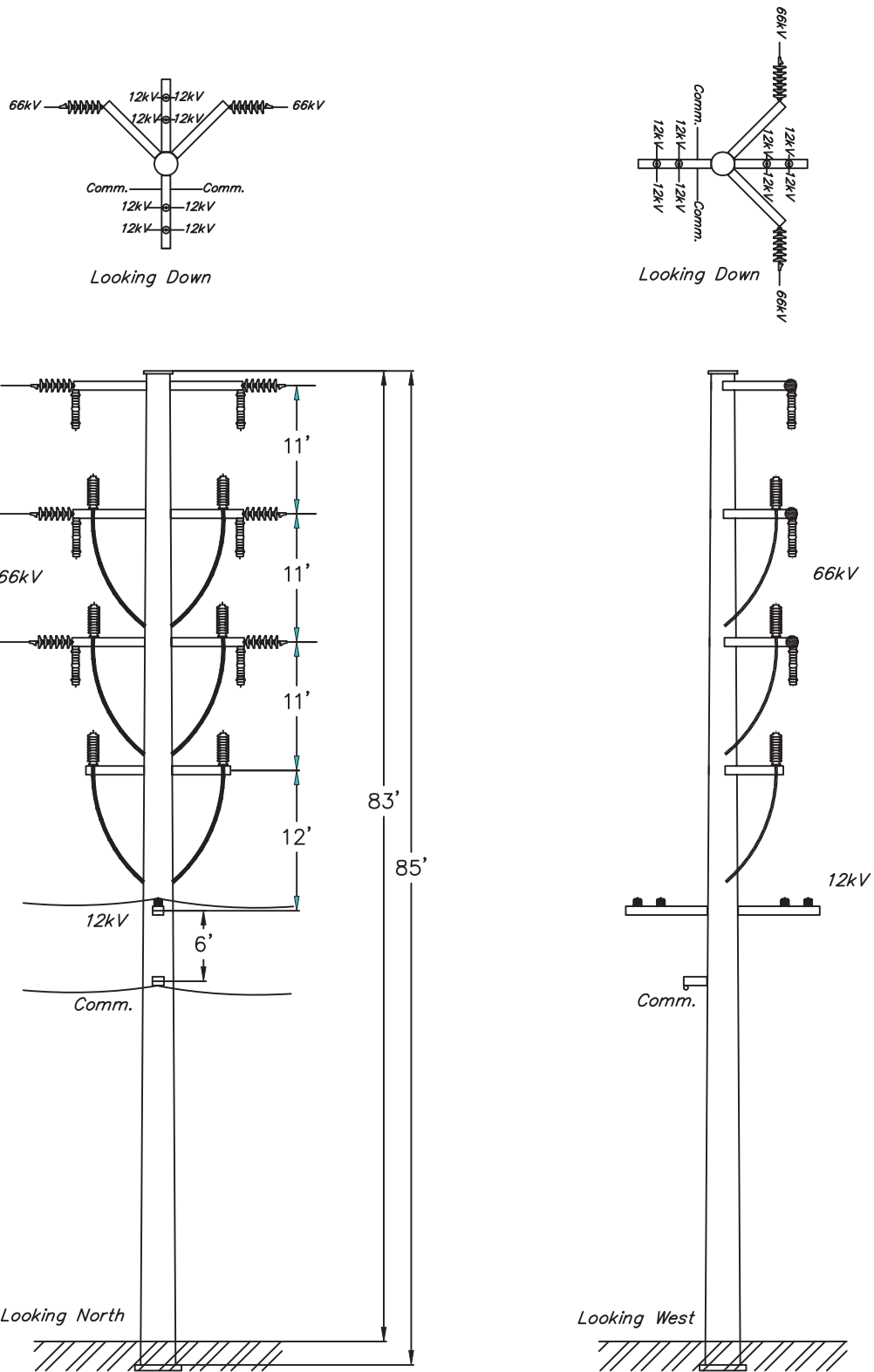
Figure B.1-8 Tubular Steel Pole for Transition to Underground Subtransmission Route
