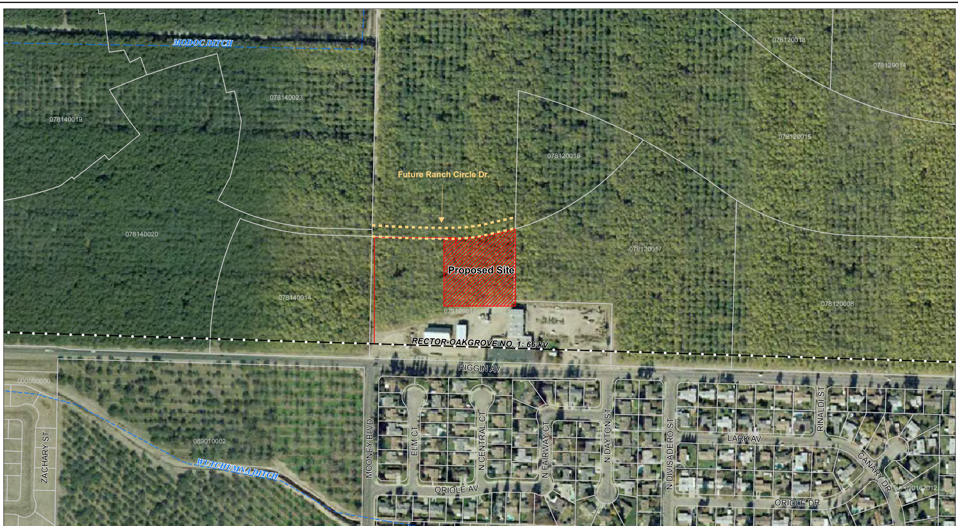
Riverway Substation Project Figure 3-1 Proposed Substation Site and Subtransmission Route
