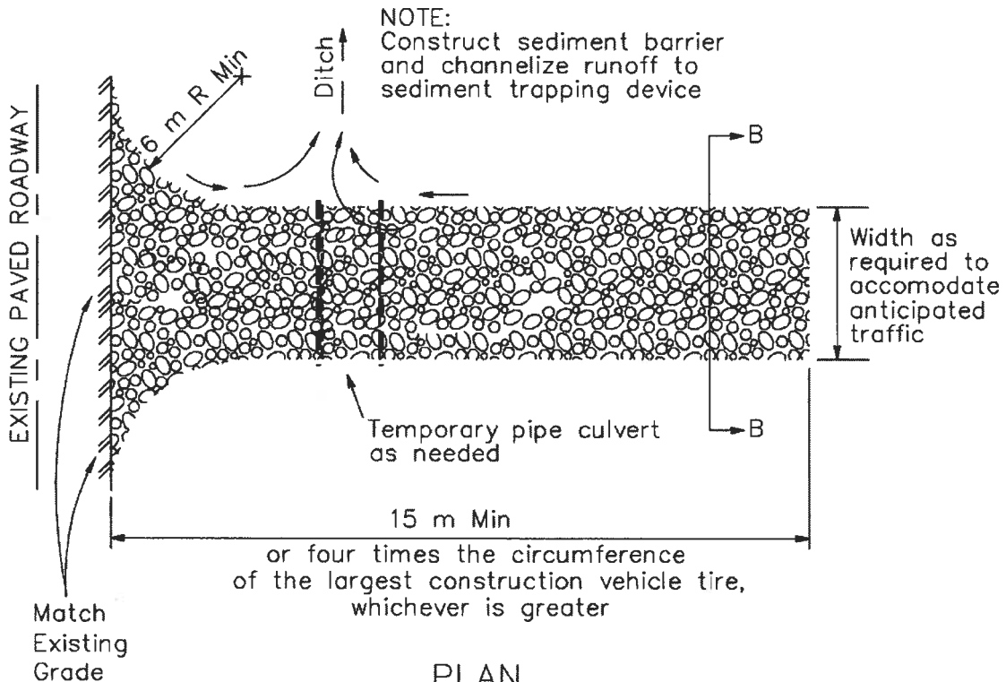
PLAN NTS
