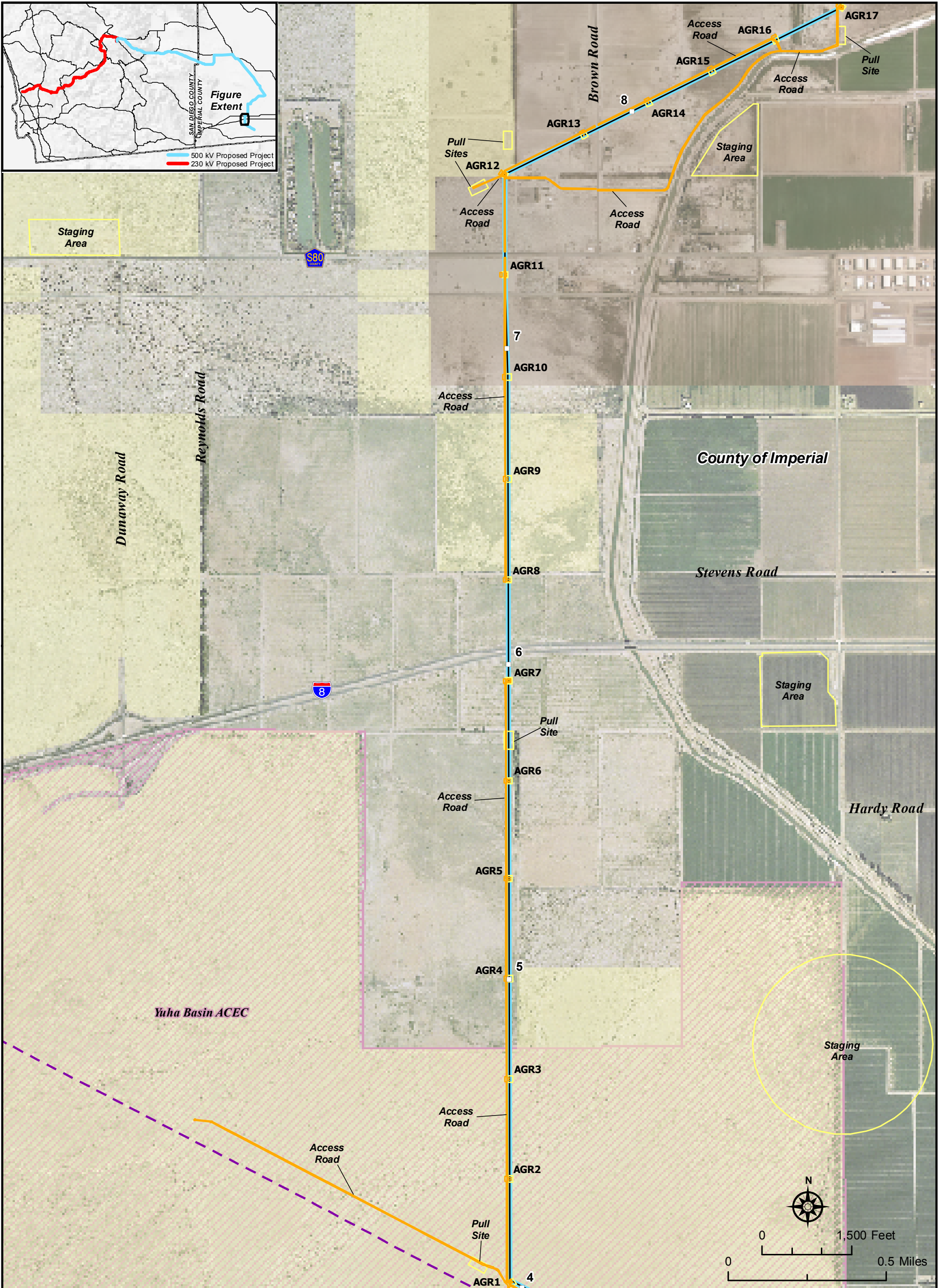
Sunrise Powerlink Project Figure Ap. 11A-3 Proposed Project Detail
