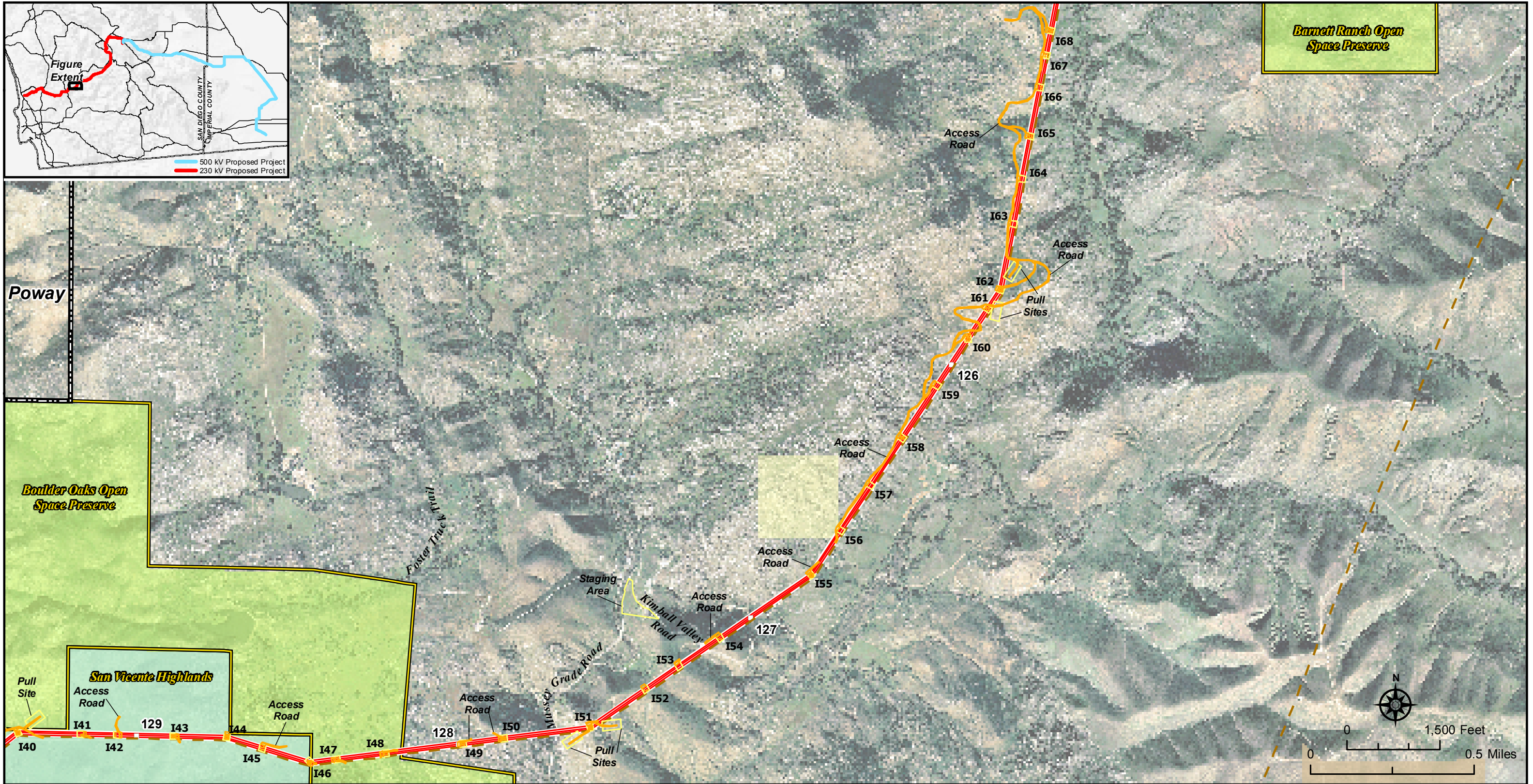
Sunrise Powerlink Project Figure Ap. 11A-31 Proposed Project Detail
