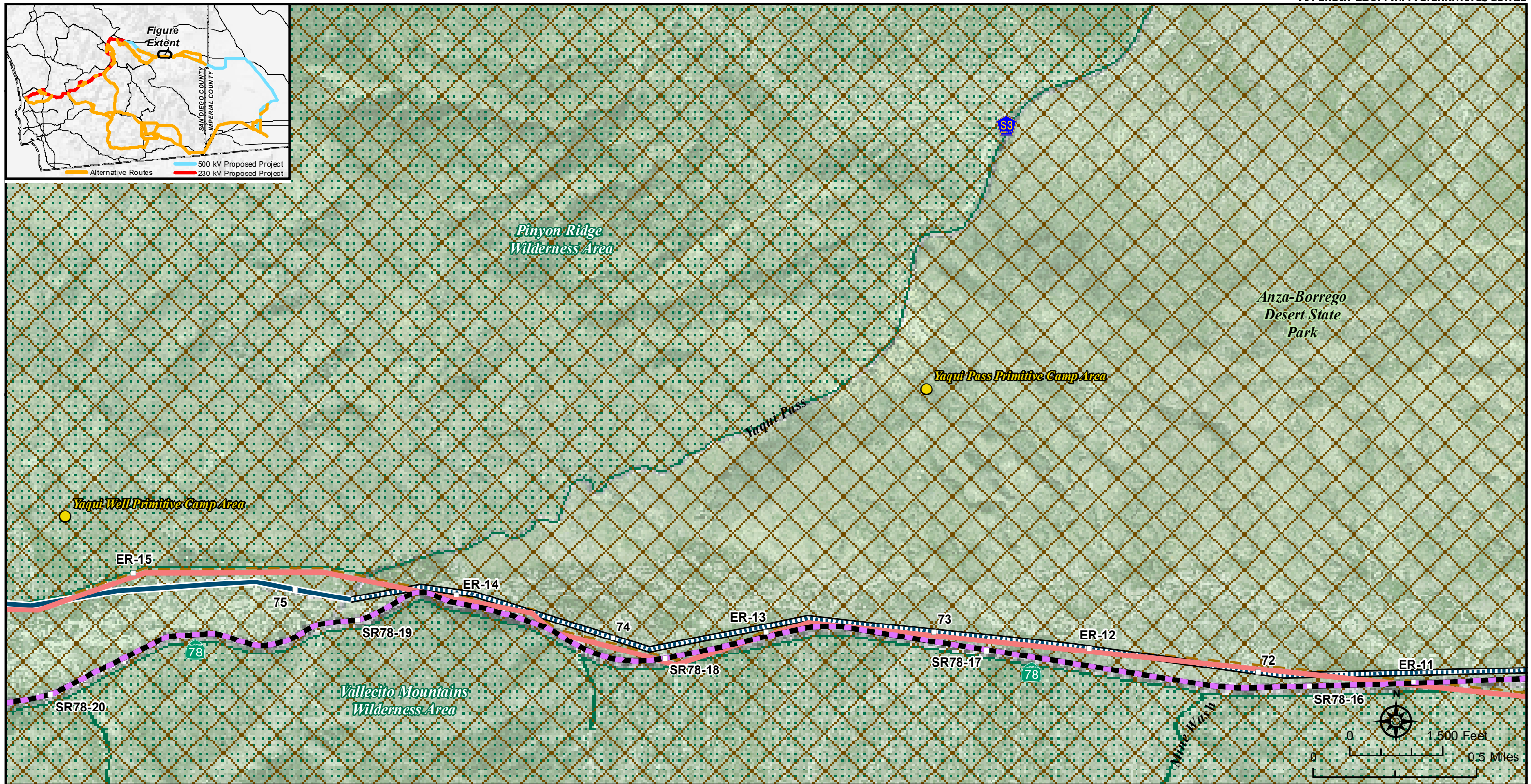
Sunrise Powerlink Project Figure Ap. 11C-8 Partial Underground ABDSP SR78 to S2 Alternative Detail
