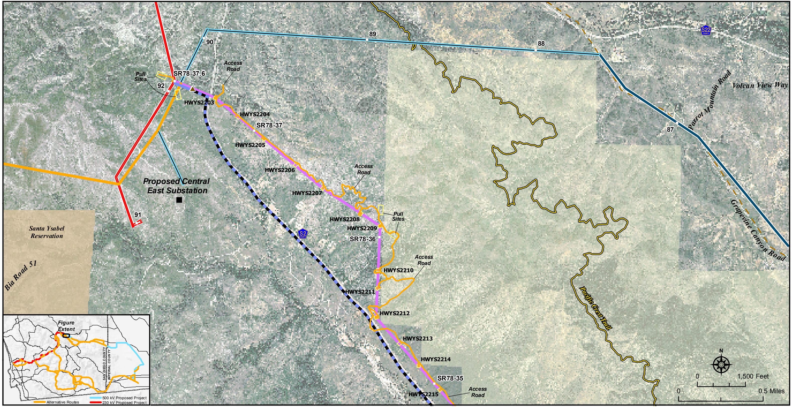
Sunrise Powerlink Project Figure Ap. 11C-13 Partial Underground ABDSP SR78 to S2 Alternative Detail
