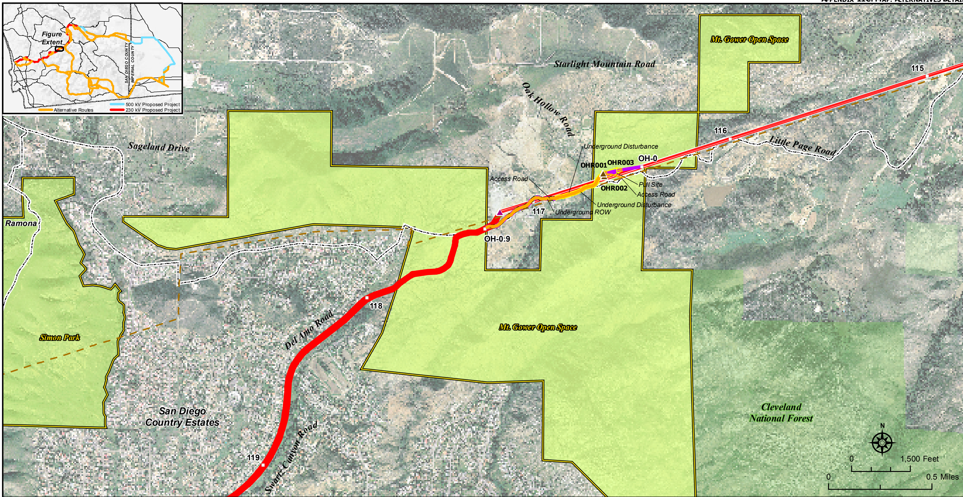
Sunrise Powerlink Project Figure Ap. 11C-26 Oak Hollow Road Underground Alternative Detail
