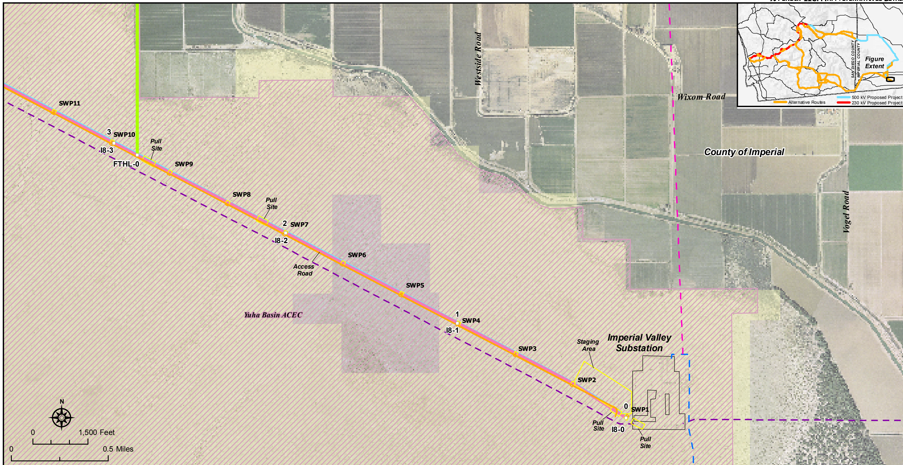
Sunrise Powerlink Project Figure Ap. 11C-35 Interstate 8 Alternative, Overhead Portion Detail
