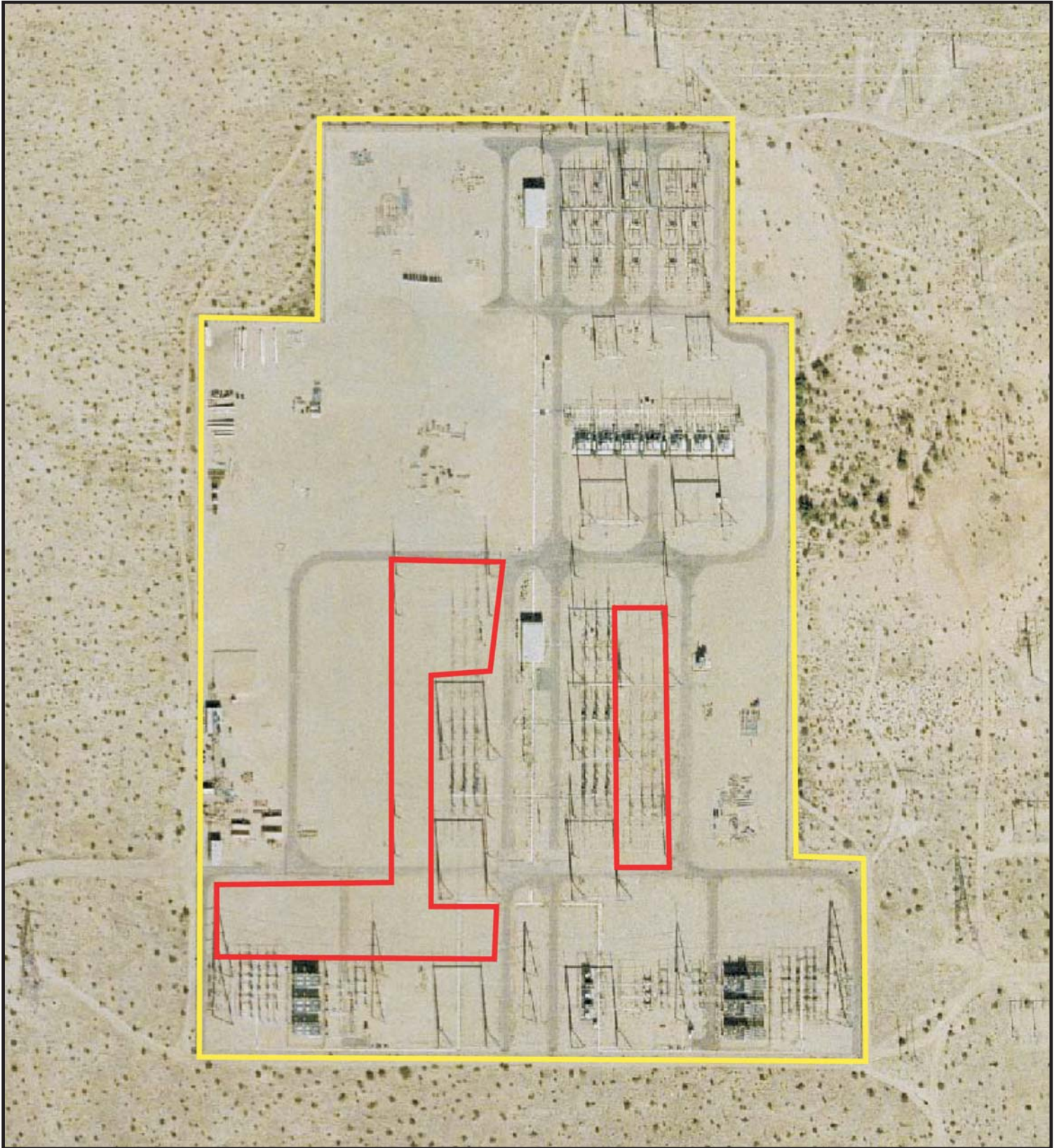
Figure B-30 Imperial Valley Substation: Proposed Modifications
