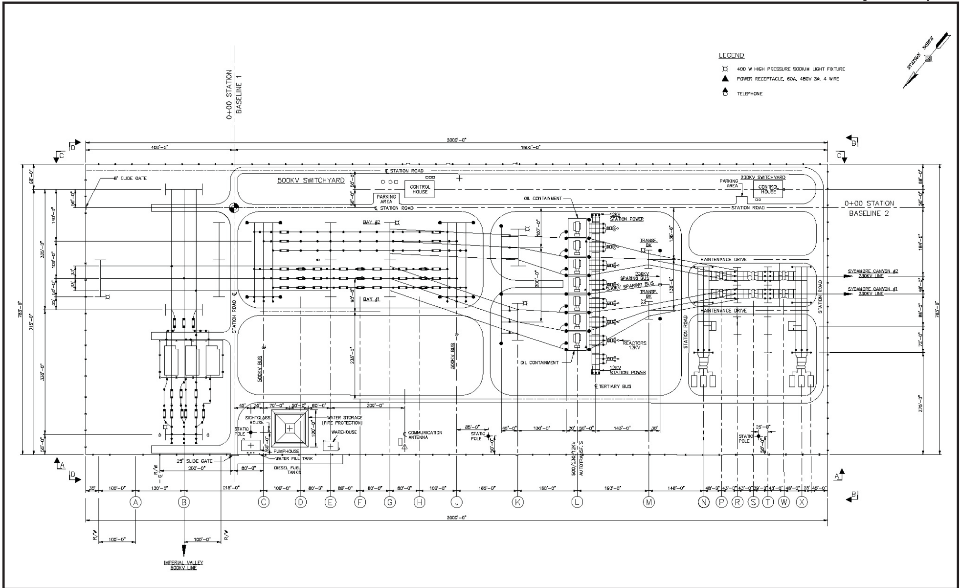
Sunrise Powerlink Project Figure B-32 Central East Substation: 500/230 kV Switchyard: General Arrangement
