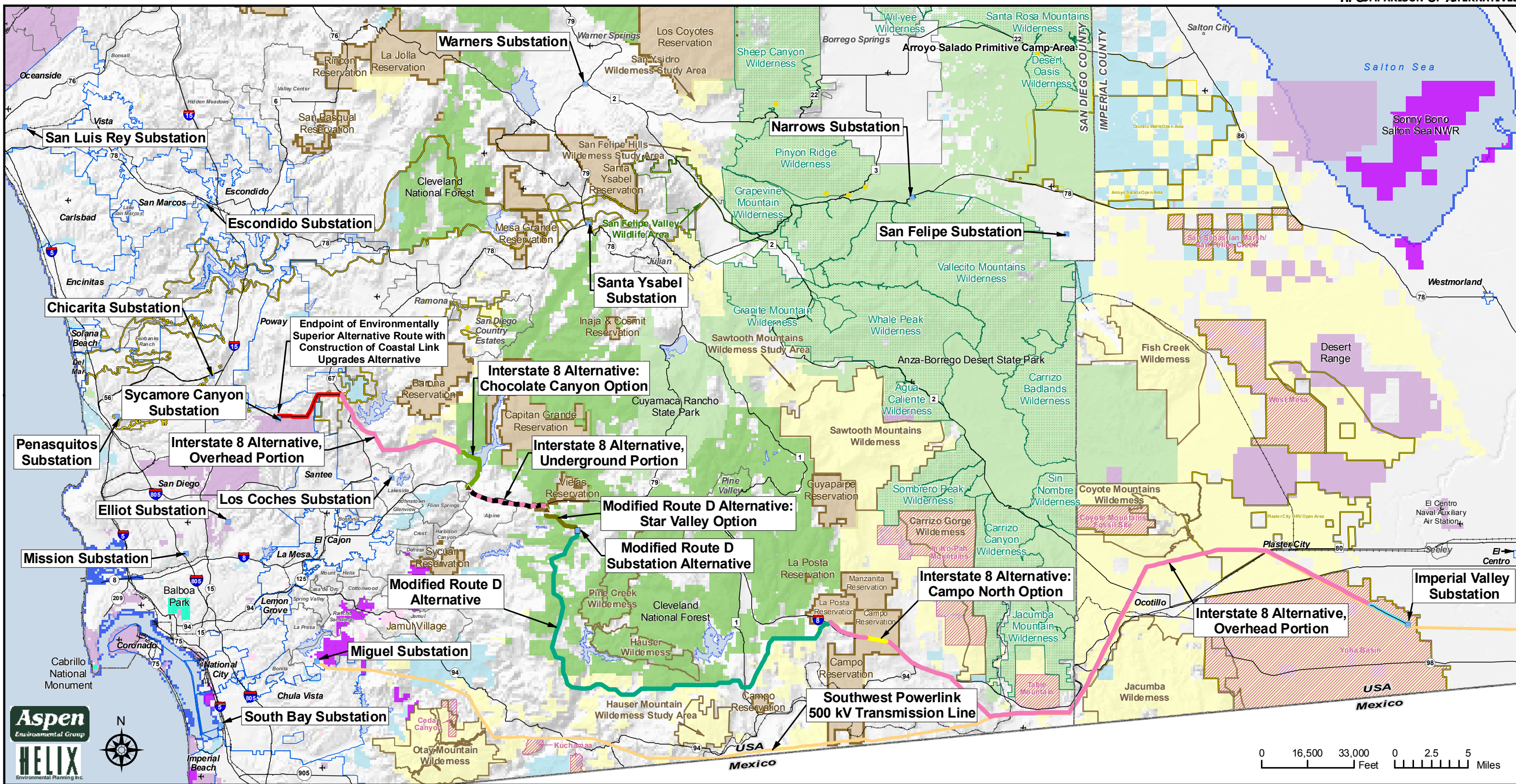
Sunrise Powerlink Project Figure H-2 Environmentally Superior SWPL Transmission Line Alternative
