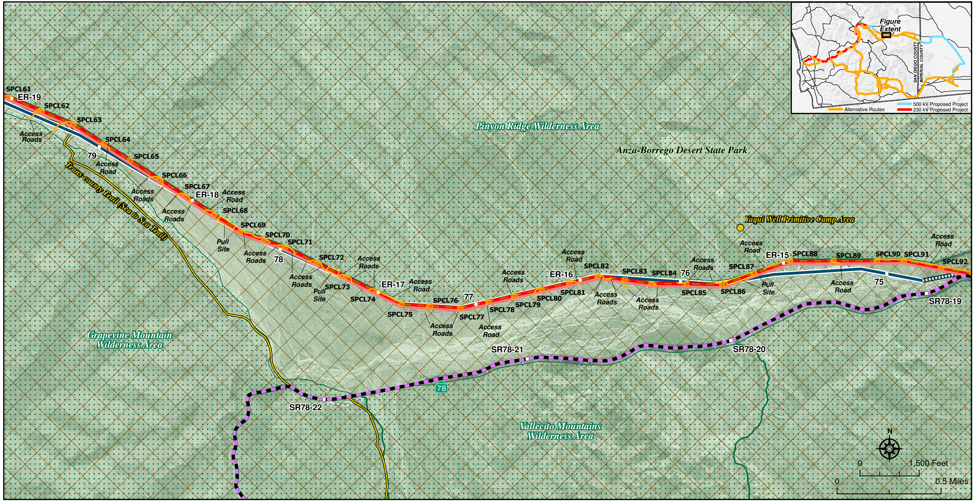
Sunrise Powerlink Project Figure Ap. 11C-17 Overhead 500 kV ABDSP Within Existing ROW Alternative Detail
