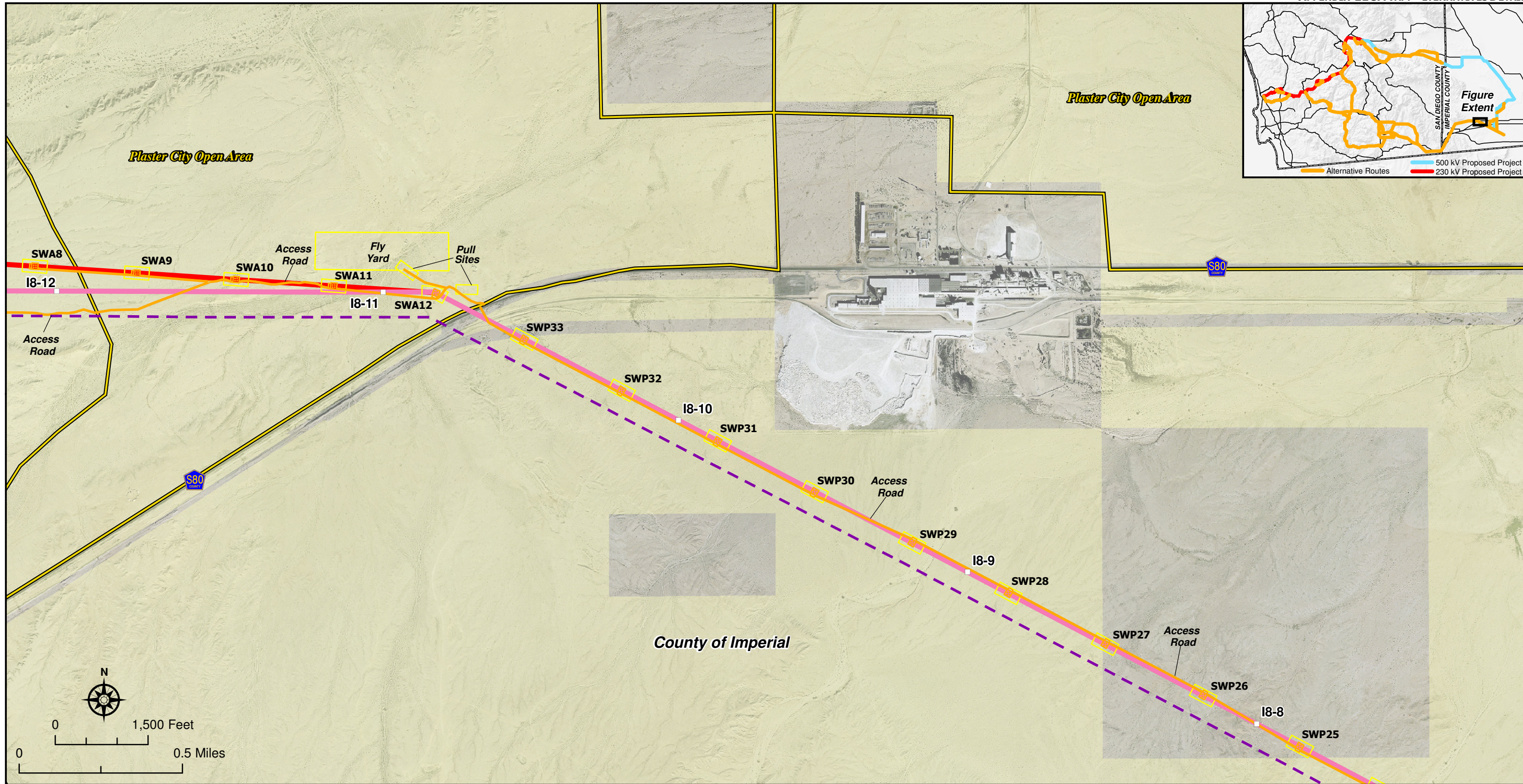
Sunrise Powerlink Project Figure Ap. 11C-37 Interstate 8 Alternative, Overhead Portion Detail
