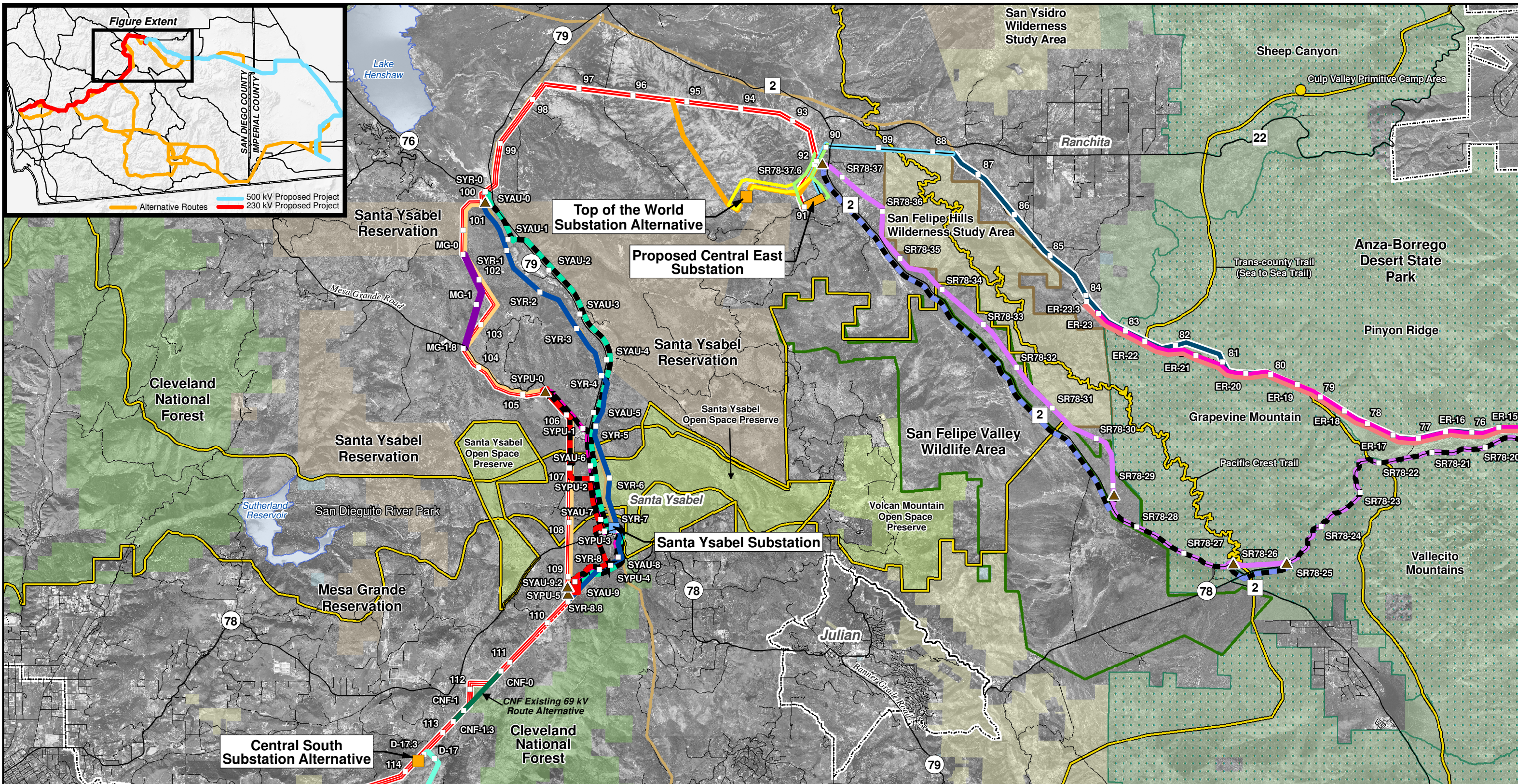
Sunrise Powerlink Project Figure ES-14 Central Link Alternatives Retained
