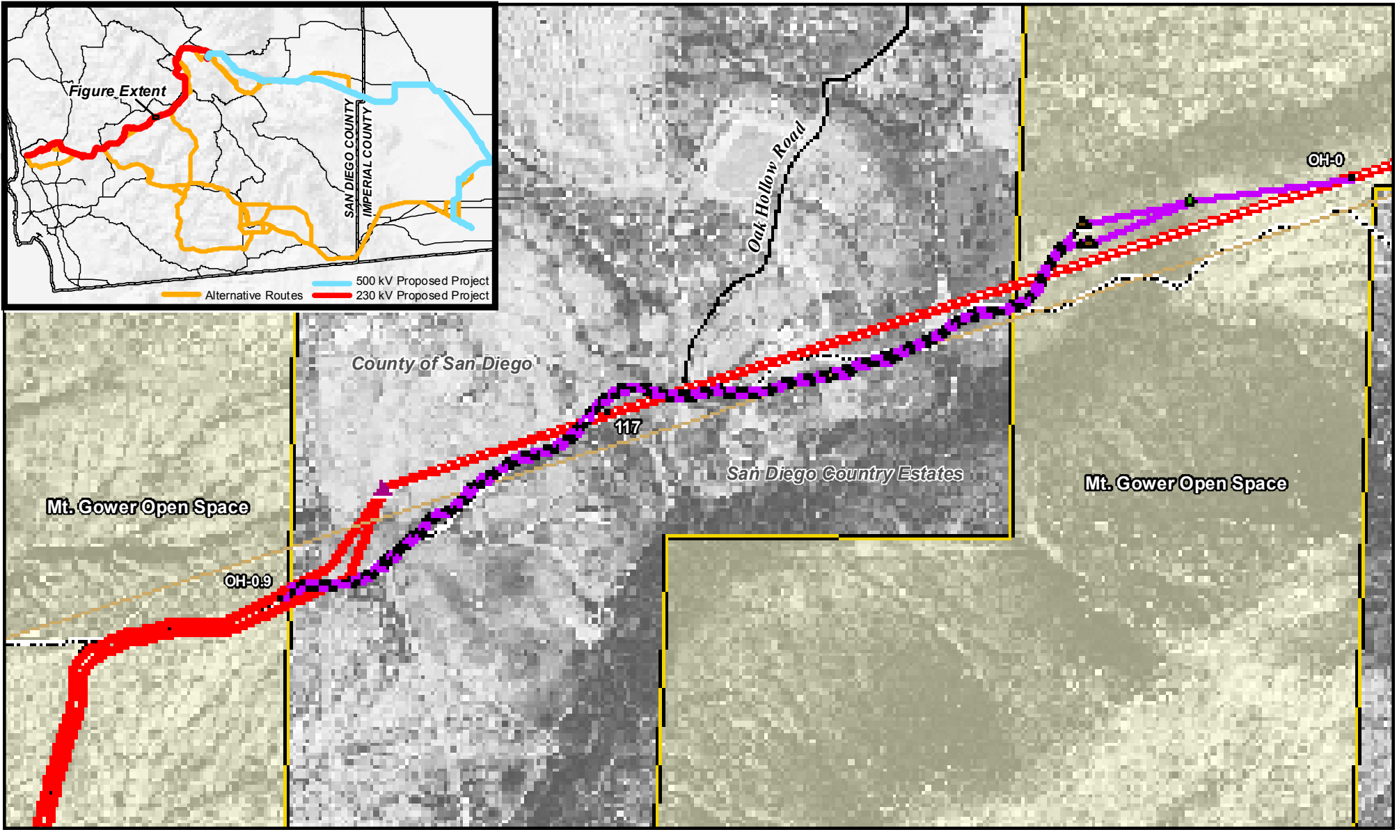
Sunrise Powerlink Project Figure D.1-6 Oak Hollow Road Underground Alternative
