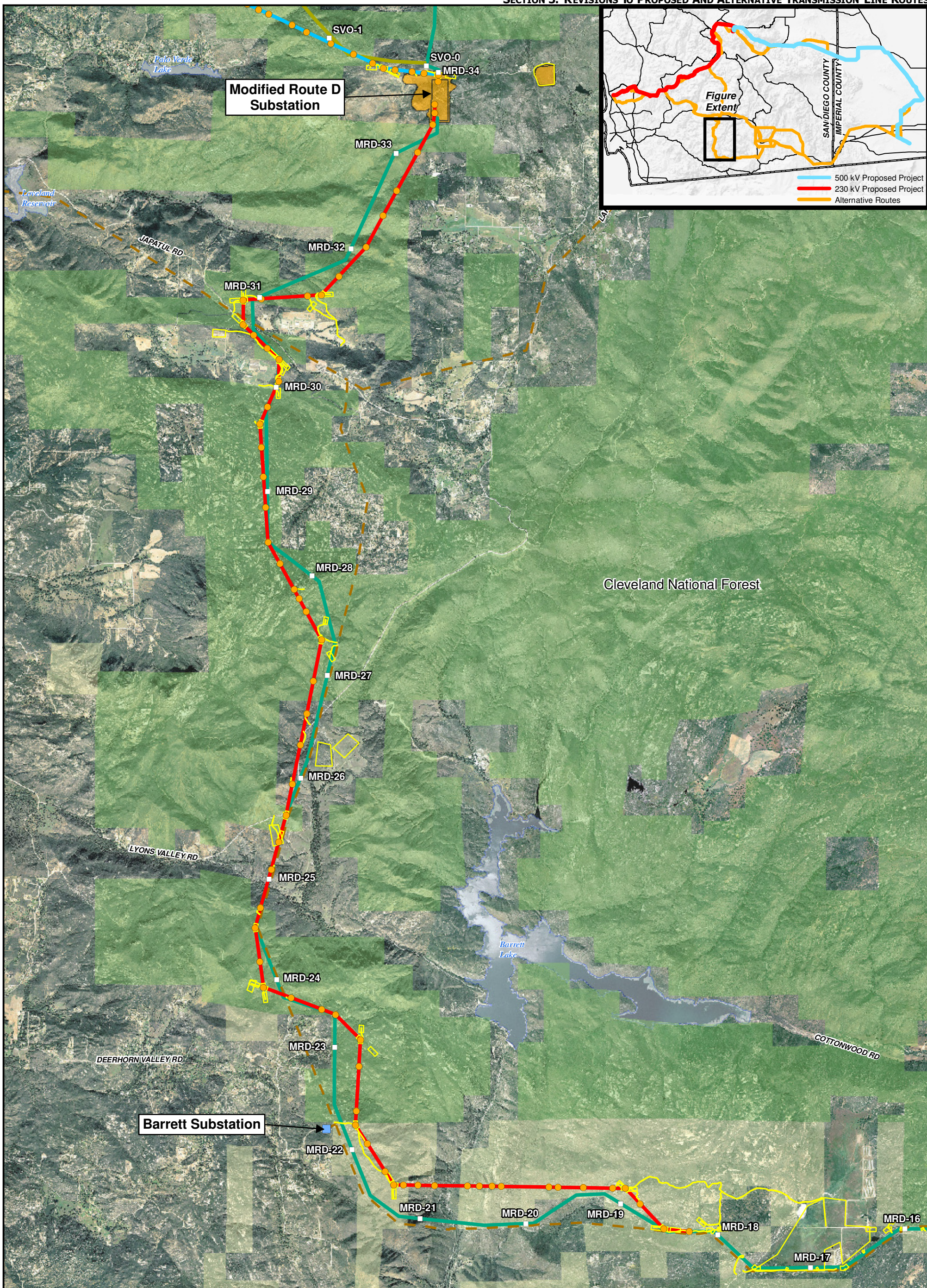
Sunrise Powerlink Project Figure 3-12 Modified Route D Alternative: Western Reroute
