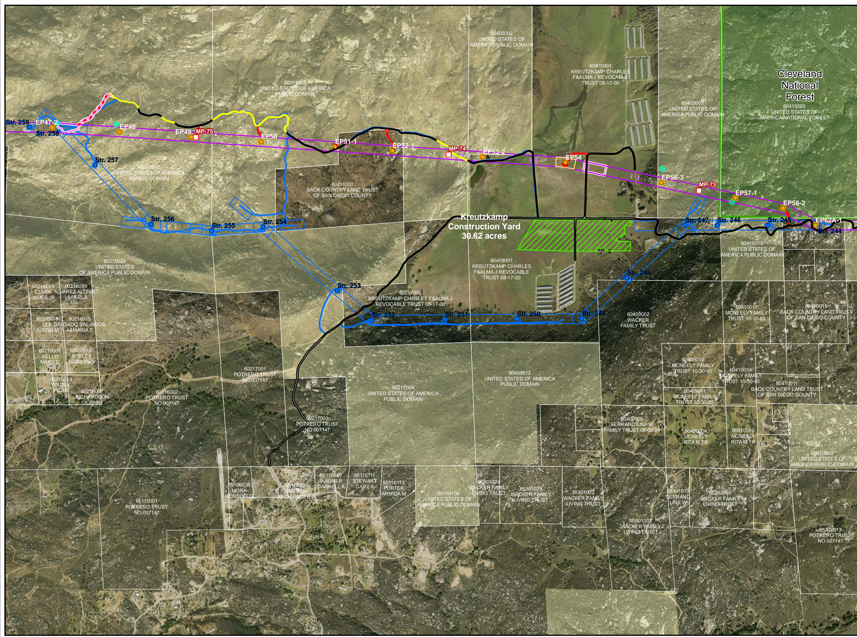
Figure 23 STRUCTURES EP62A-1 TO EP47-2 (PORTRERO)
