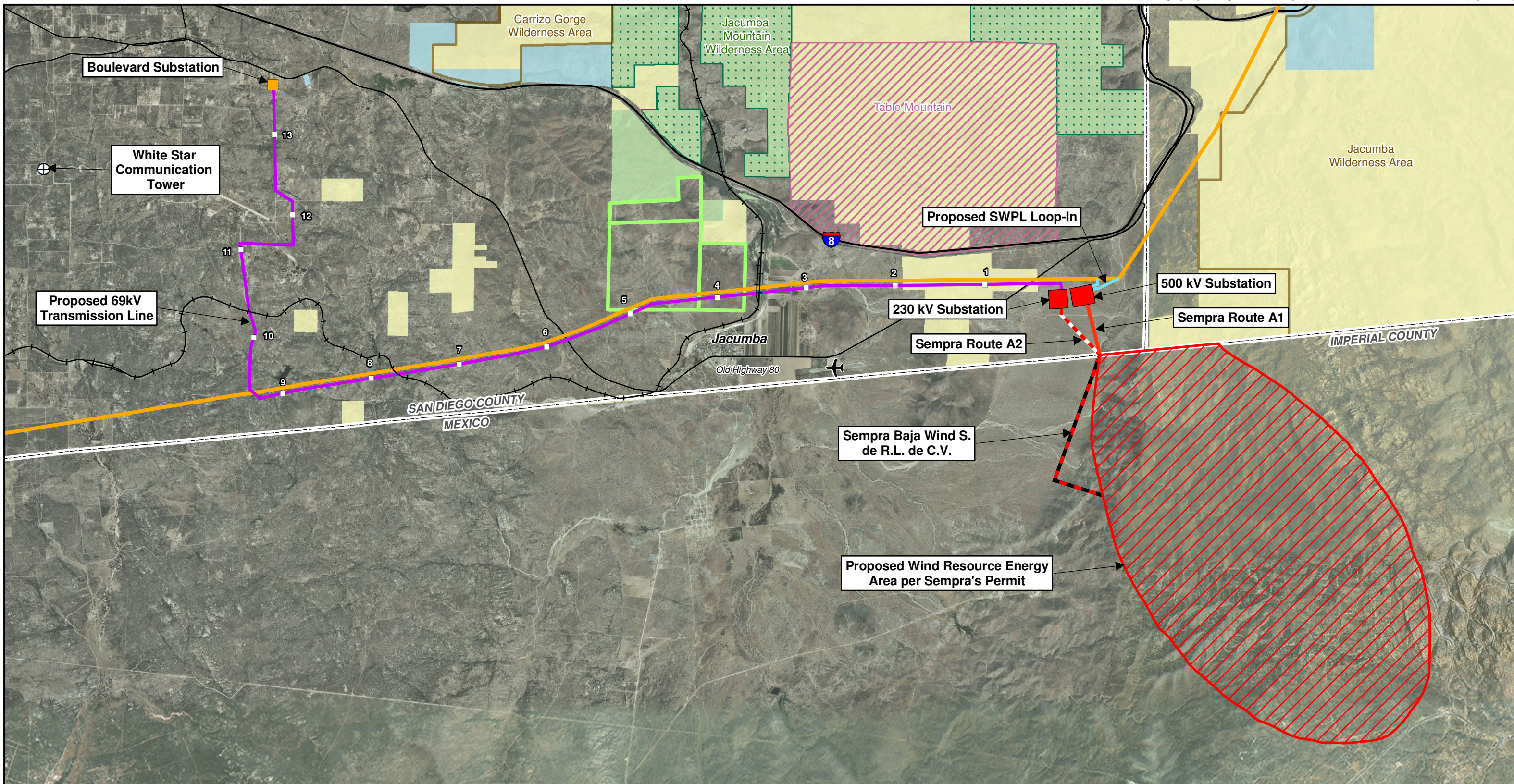
Sunrise Powerlink Project Figure 2-3 Sempra Rumorosa Wind Energy Projects and Baja Wind Transmission Recirculated Draft EIR/Supplemental Draft EIS
