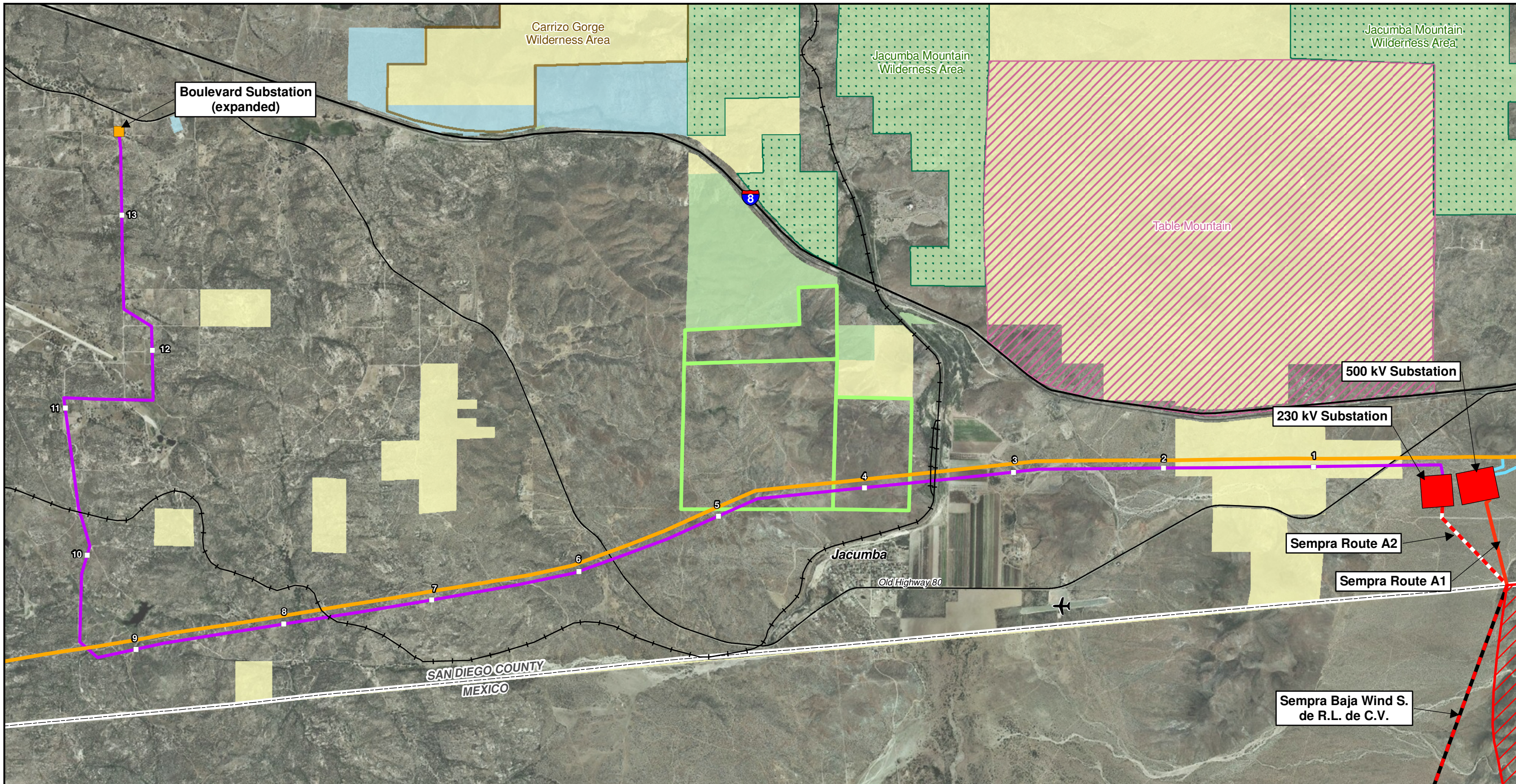
Sunrise Powerlink Project Figure 2-4 New SDG&E 69kV Transmission Line and Expanded Boulevard Substation
