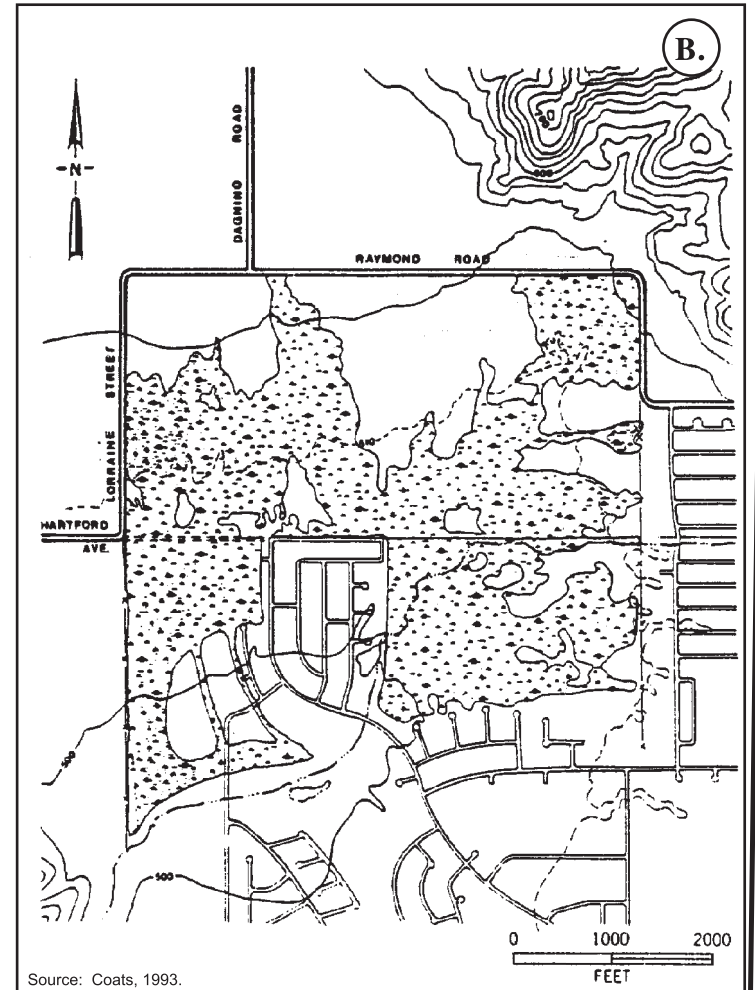
B. Springtown Alkali Sink bordered by Raymond Road and other surrounding roads.
