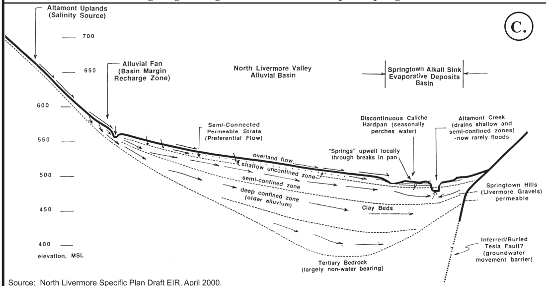
C. Cross-sectional view of geologic and groundwater relationships at Springtown Alkali Sink and areas north.
