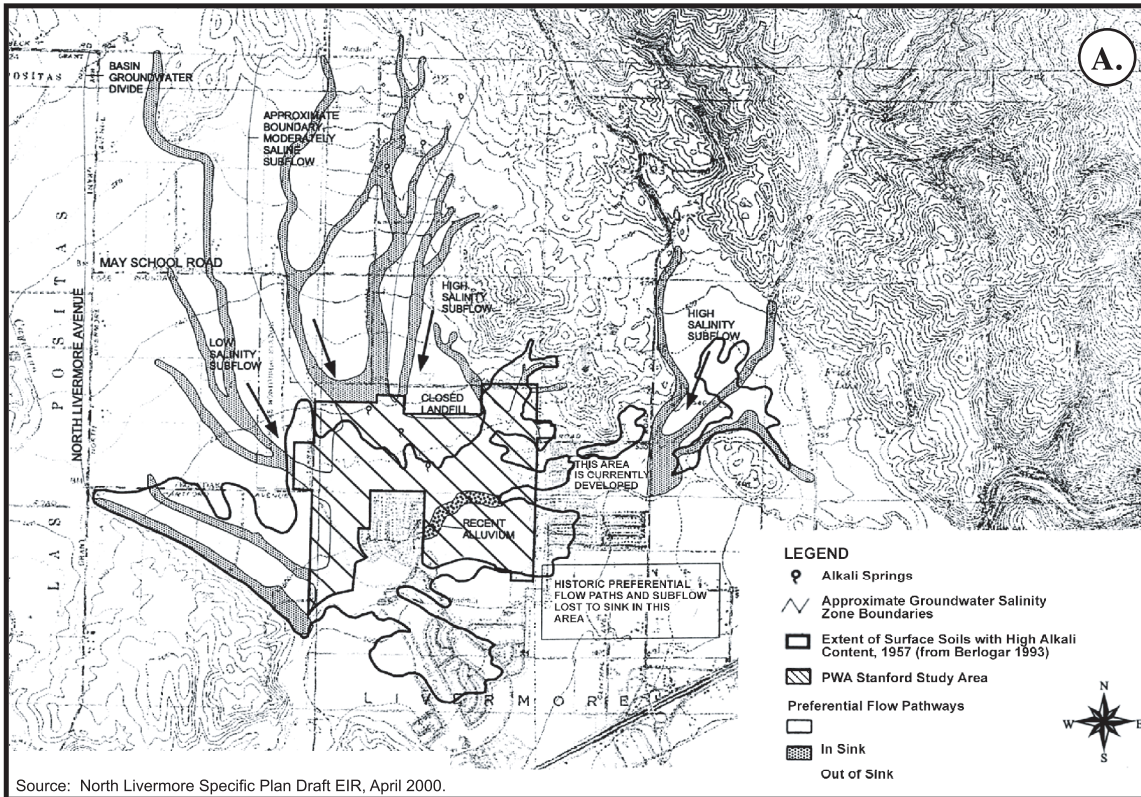
A. Preferential flow pathways supplying shallow sub-surface water to Springtown Alkali Sink.
