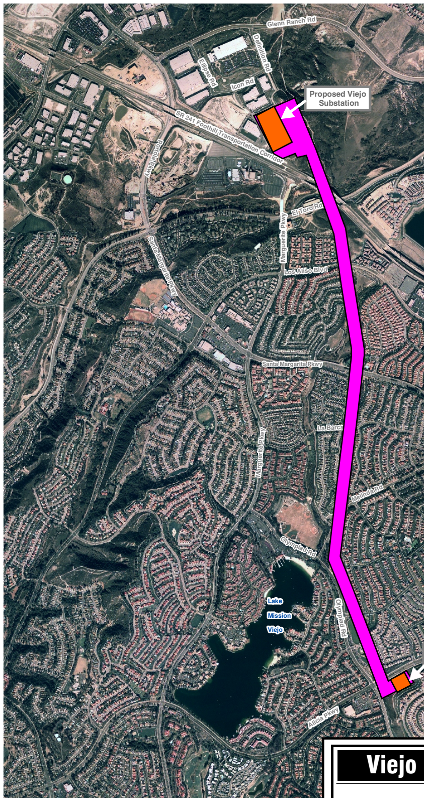
Figure 2 Proposed Substation Site and 66 kV Subtransmission Line Route
