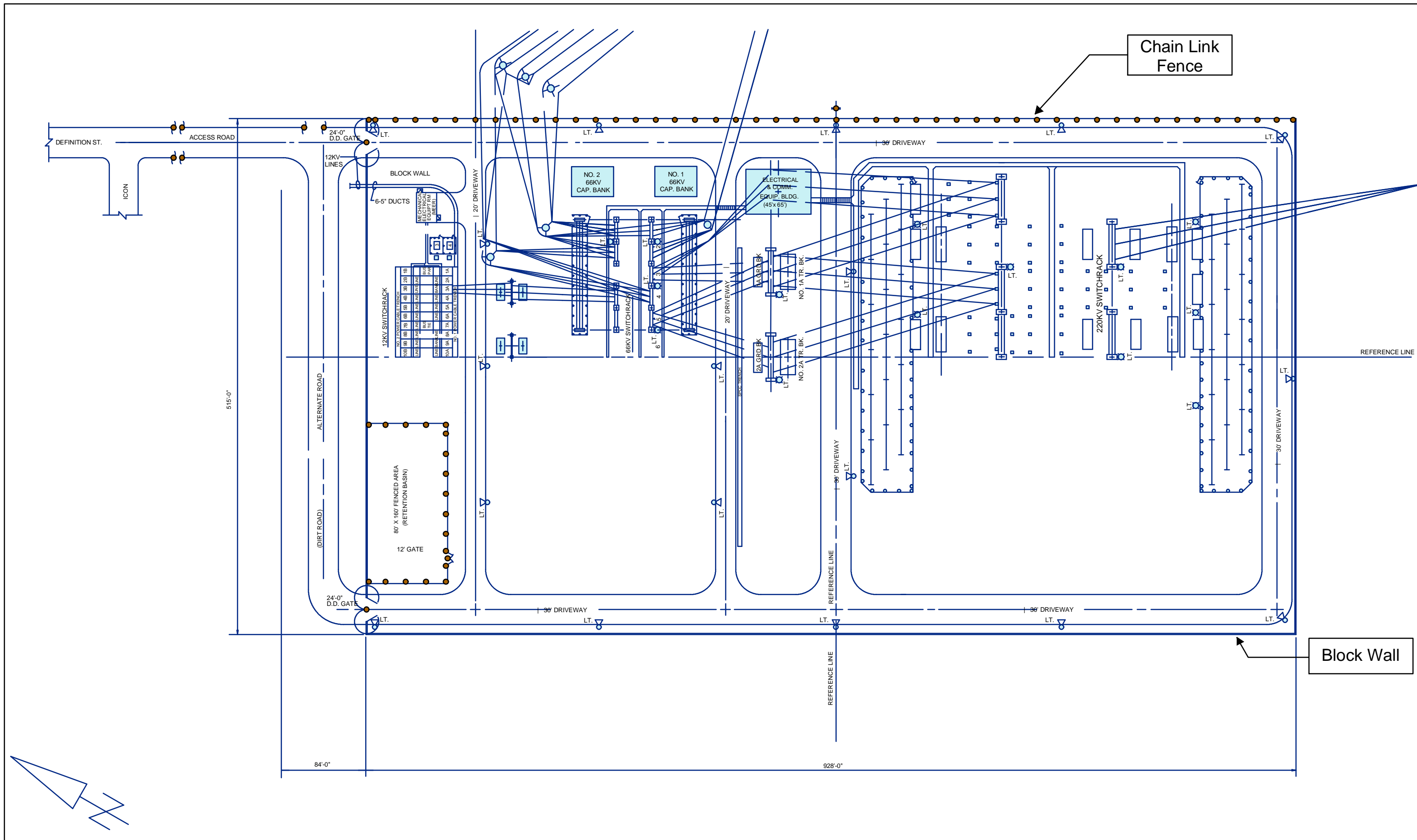
Proposed Viejo Substation Site Plan
