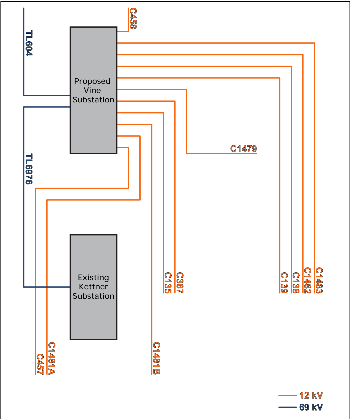
Figure B.1-6: Proposed System Configuration
