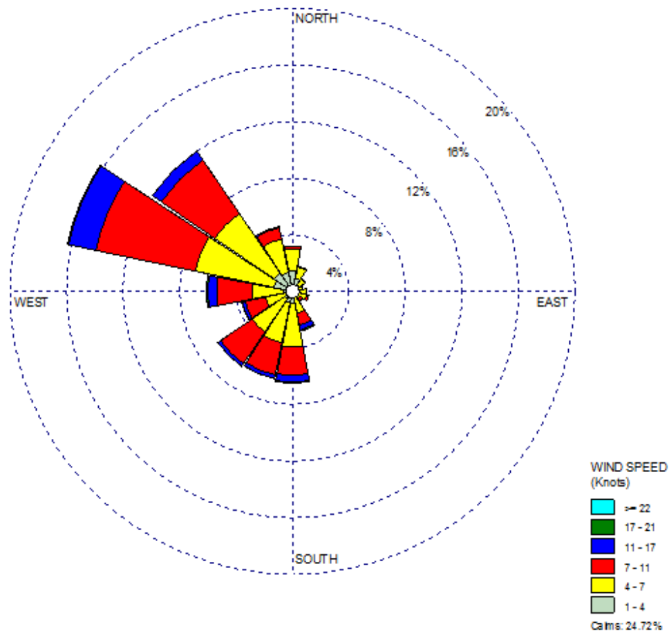
Figure B.3.3-1 – Windrose from San Diego International Airport (2009 – 2013)
