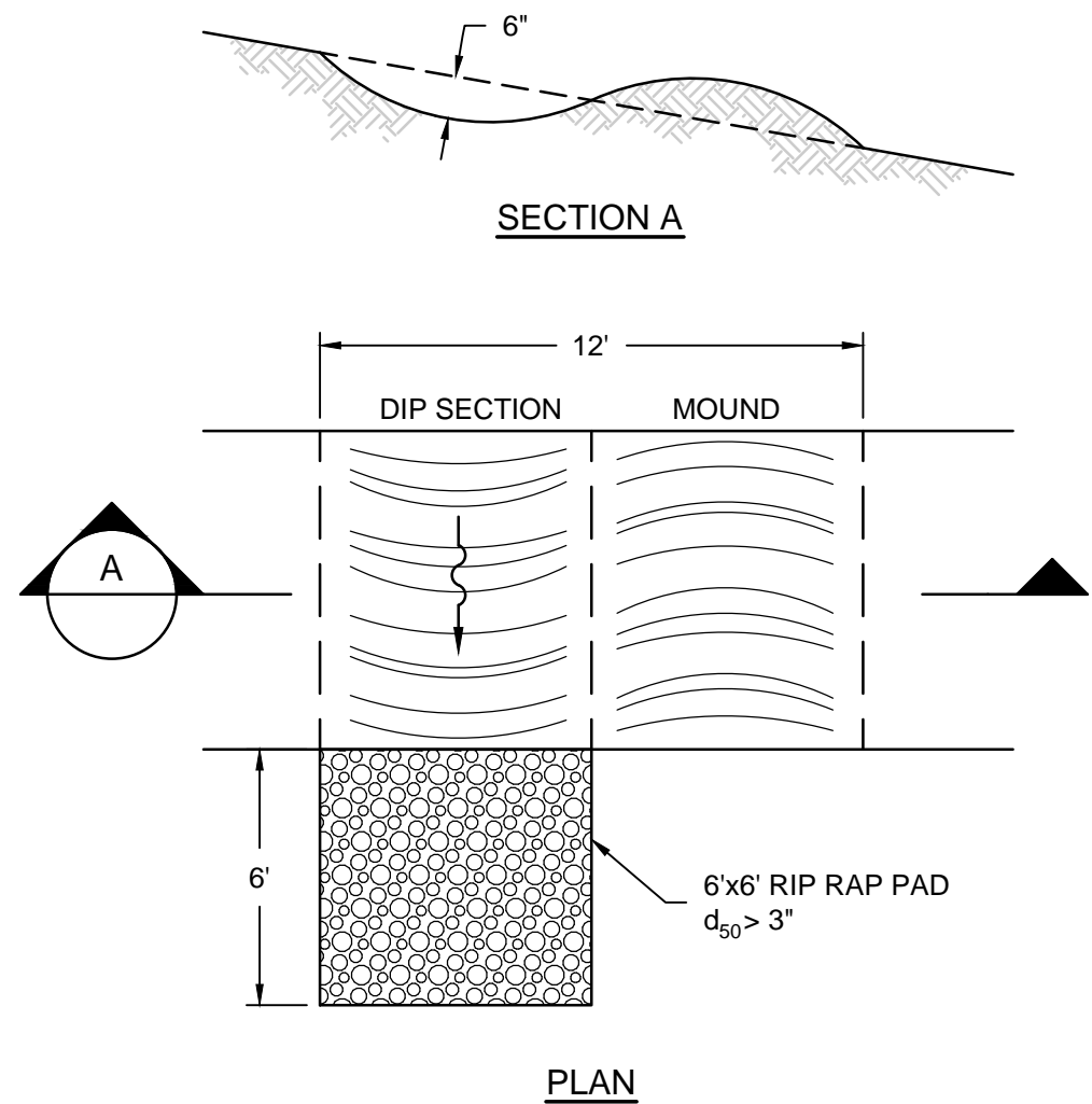
3 2 DETAIL WATER BAR WITH ENERGY DISSIPATOR NTS XREF: SC0625-ECO-X08 DET water bar.dwg
