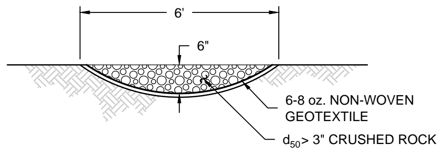
4 2 DETAIL DIP SECTION CROSSING NTS XREF: SC0625-ECO-X09 DET dip section.dwg
