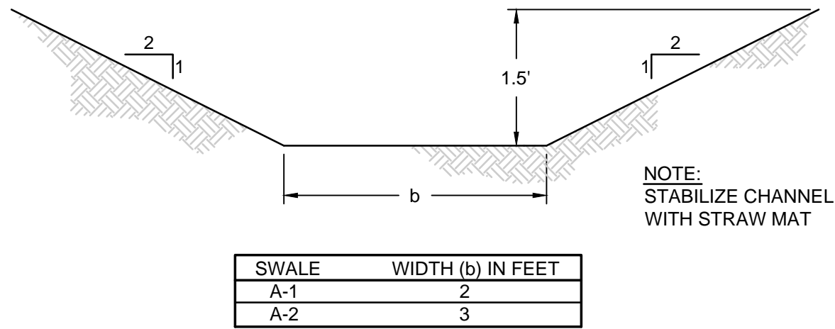
1 2,3 DETAIL DRAINAGE SWALE NTS XREF: SC0625-ECO-X06 DET swale.dwg
