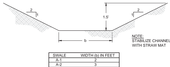
1 2,3 DETAIL DRAINAGE SWALE NTS XREF: SC0625-ECO-X06 DET swale.dwg
