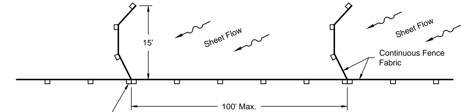
7 3,6 DETAIL SILT FENCE J-HOOKS NTS XREF: SC0625-ECO-X12 DET J-hook.dwg
