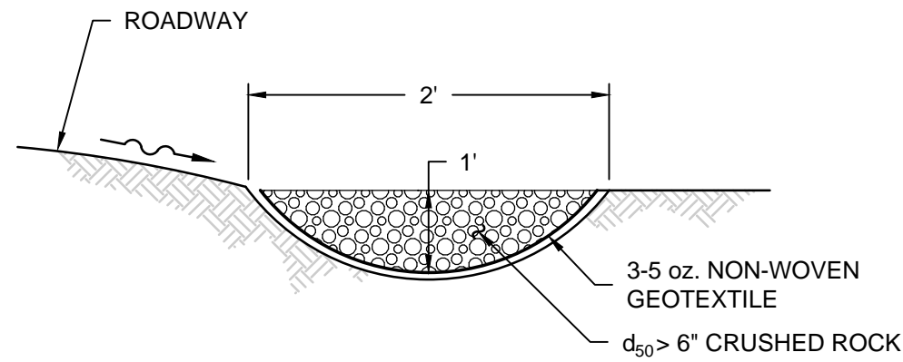
5 2,3 DETAIL ROCK-LINED SWALE NTS XREF: SC0625-ECO-X10 DET rock-lined swale.dwg
