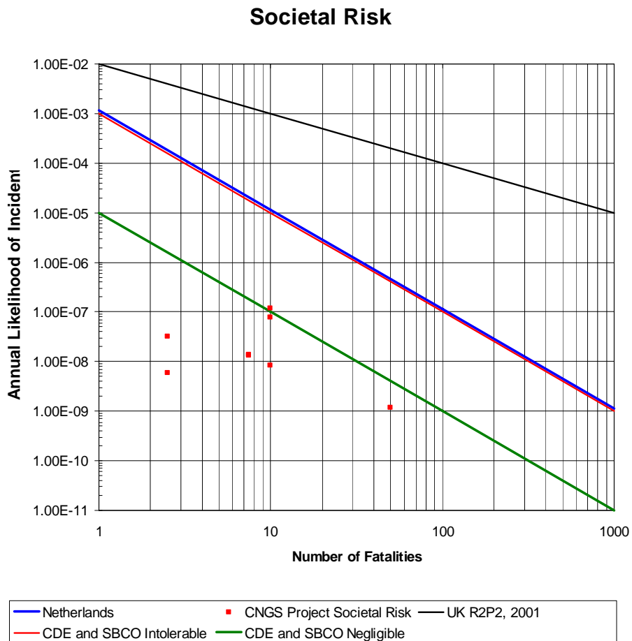
Figure 6.7.3-1 Societal Risk Results
