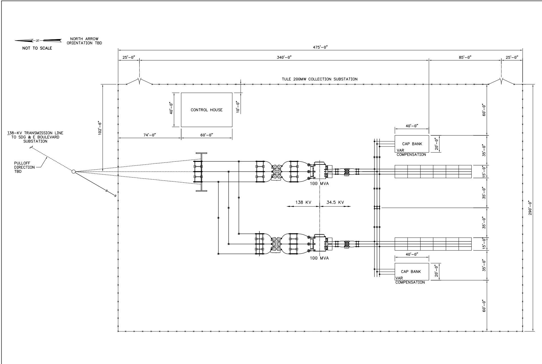
FIGURE B-27 Tule Wind Project Plan View of a Typical Collector Substation
