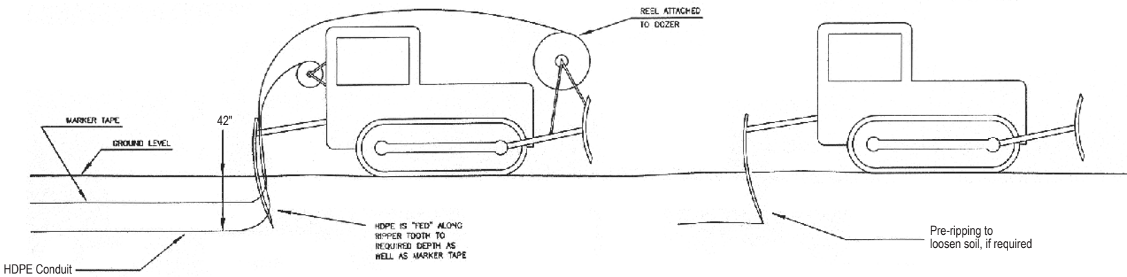
DIRECT BURIED/TRENCH HDPE PLOW METHOD
