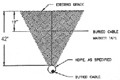
DIRECT BURIED/TRENCH HDPE PLOW METHOD
