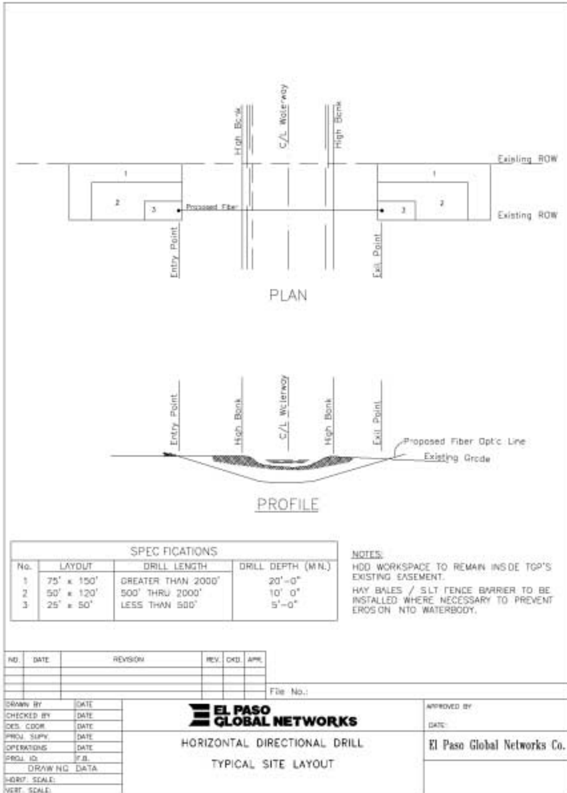
Figure 2.4-2. Standard Directional Bore Operation
