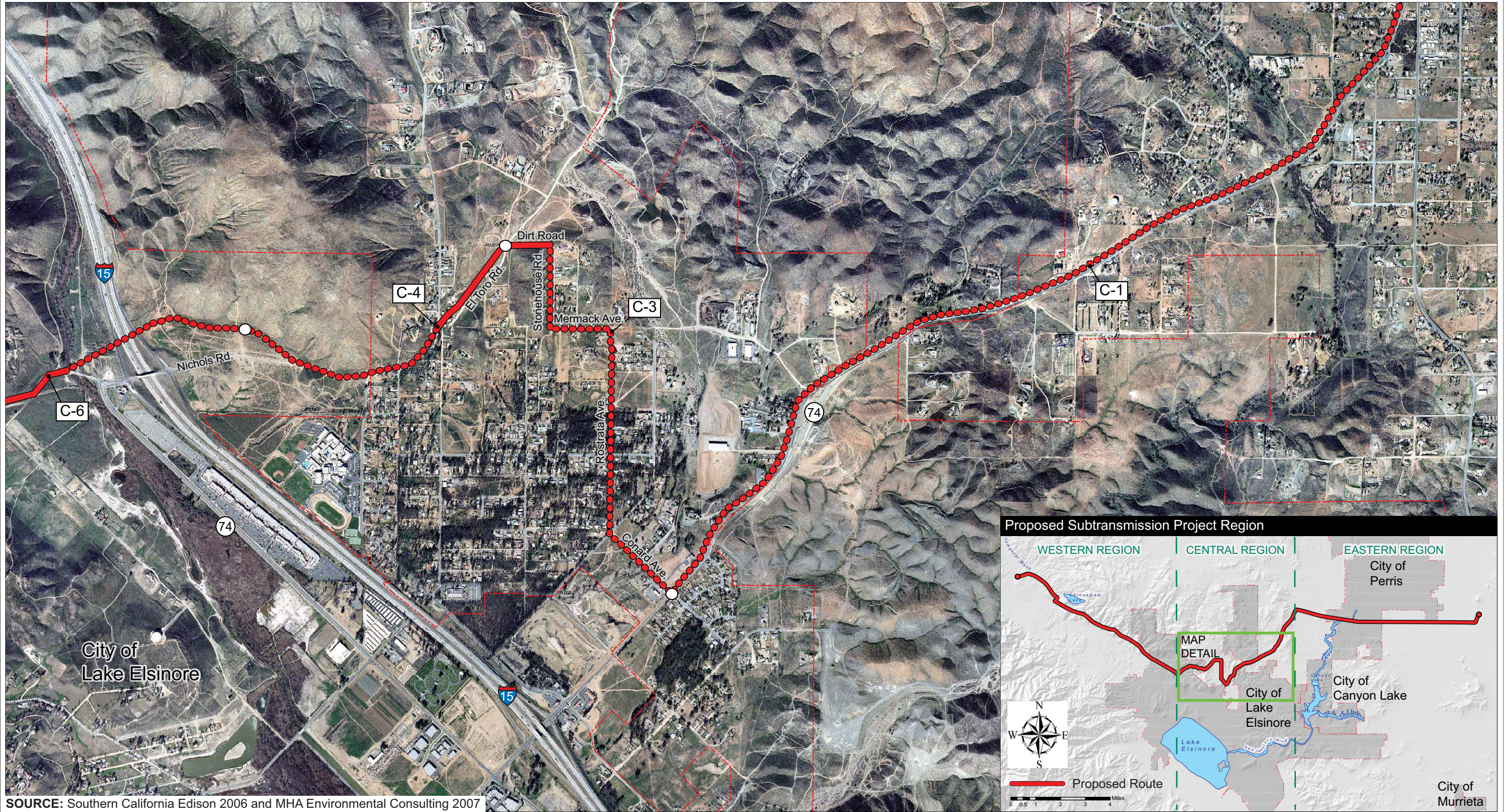
Figure B.3-4 Proposed Subtransmission Route Segments C-3, C-4 and C-6
