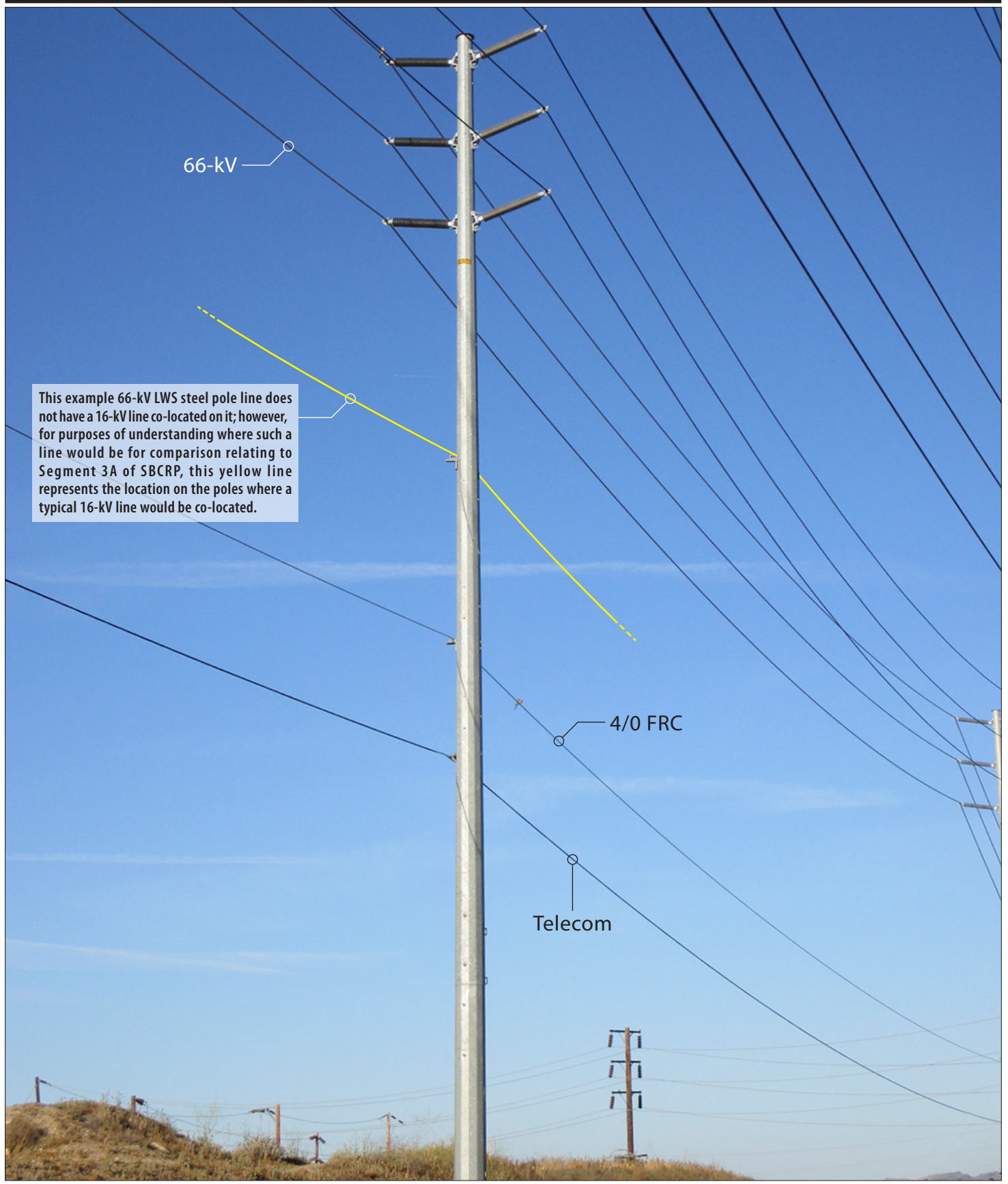
Figure 2-5 Example Fault Return Conductor
