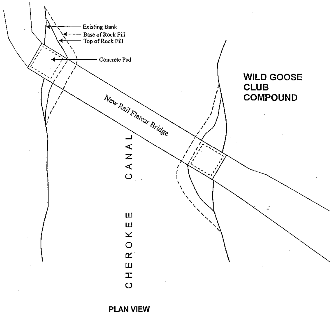
Figure 4 (Revised) ACCESS BRIDGE Wild Goose Gas Storage Project Butte County, CA
