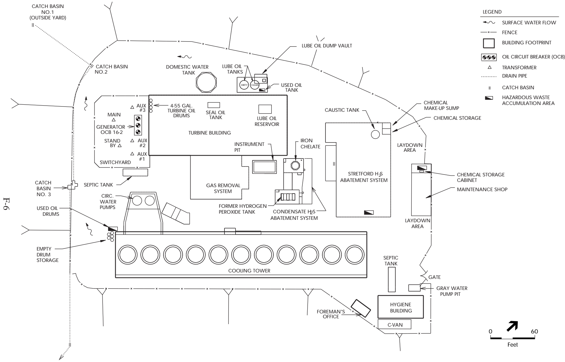
Figure F.6 Facility Layout Map for Unit 16
