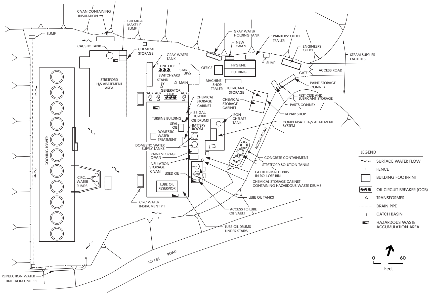
Figure F.7 Facility Layout Map for Unit 17
