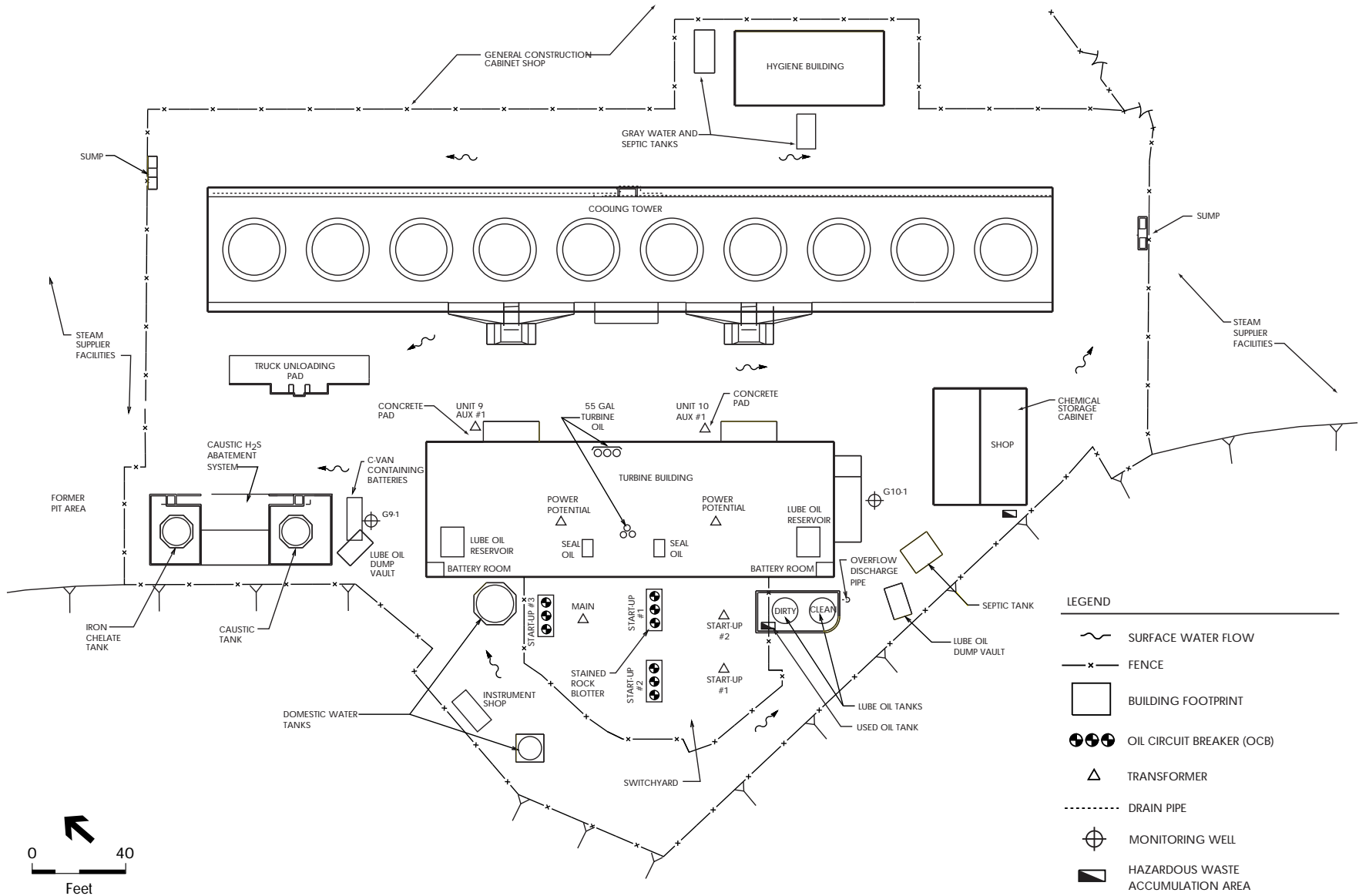
Figure F.3 Facility Layout Map for Units 9 and 10
