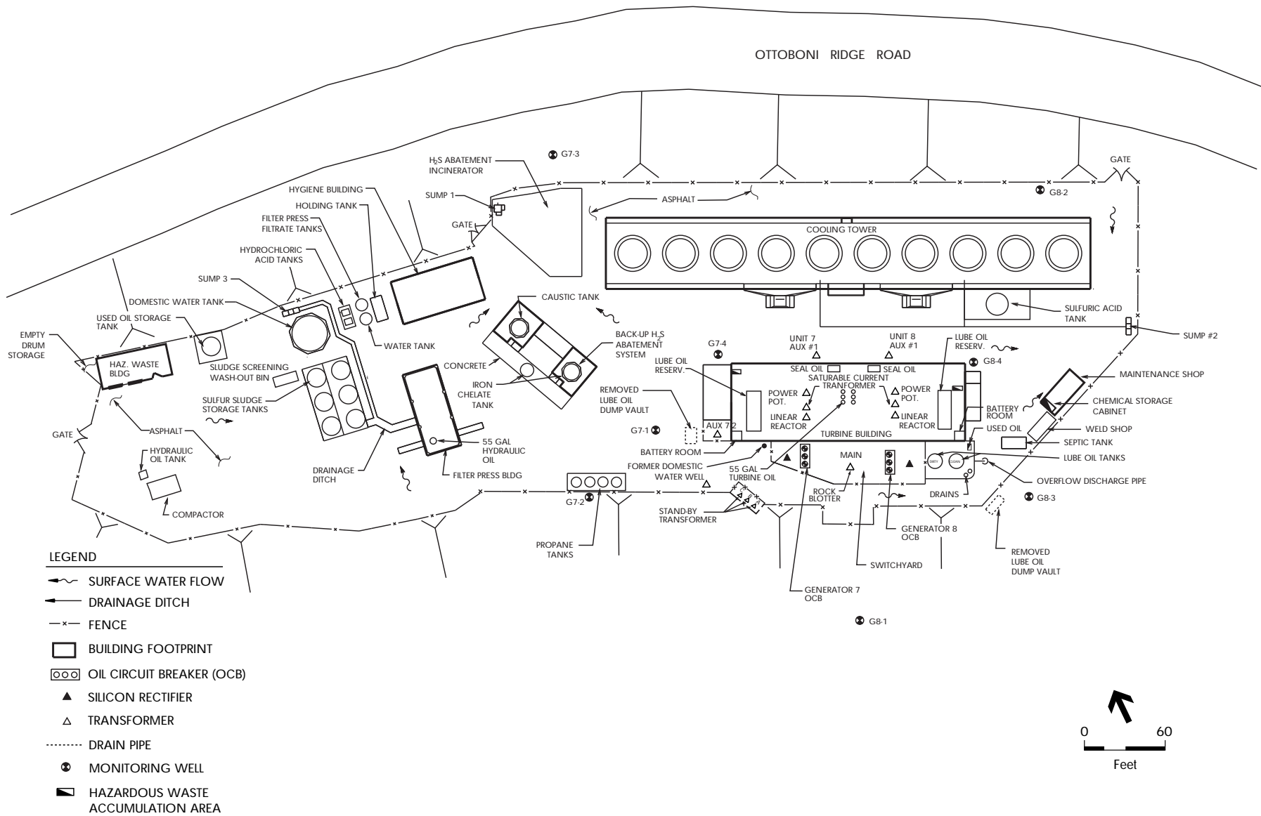
Figure F.2 Facility Layout Map for Units 7 and 8
