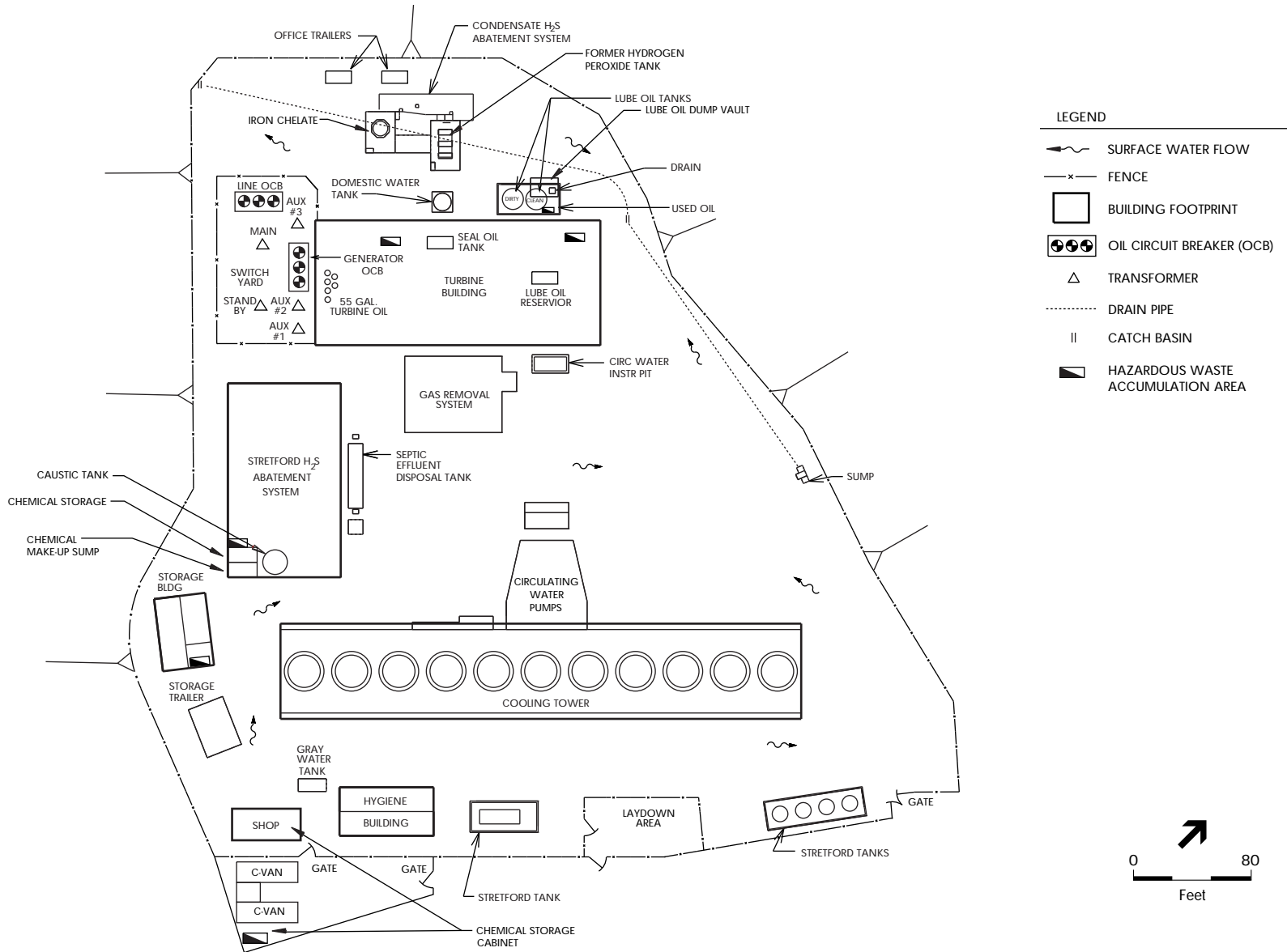
Figure F.8 Facility Layout Map for Unit 18
