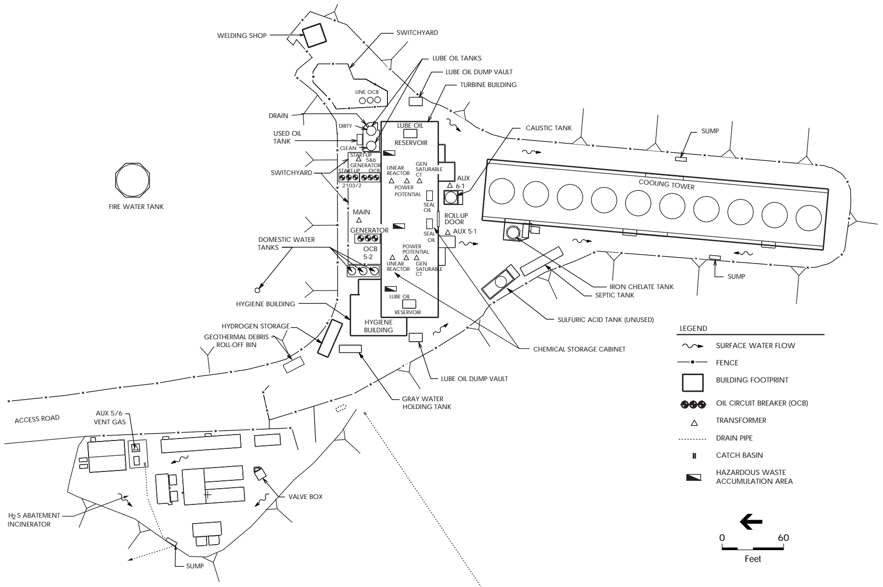
Figure F.1 Facility Layout Map for Units 5 and 6
