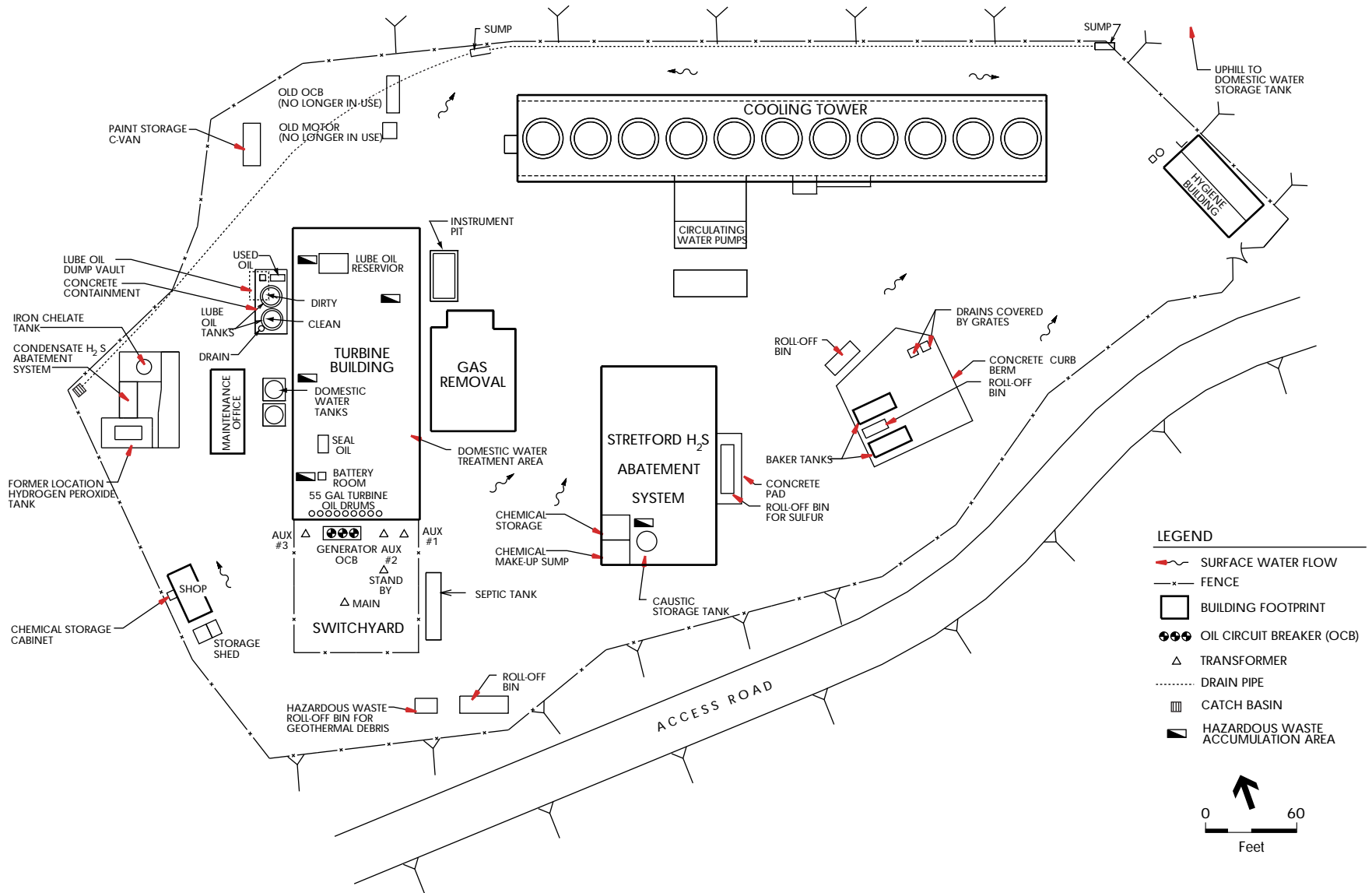
Figure F.9 Facility Layout Map for Unit 20
