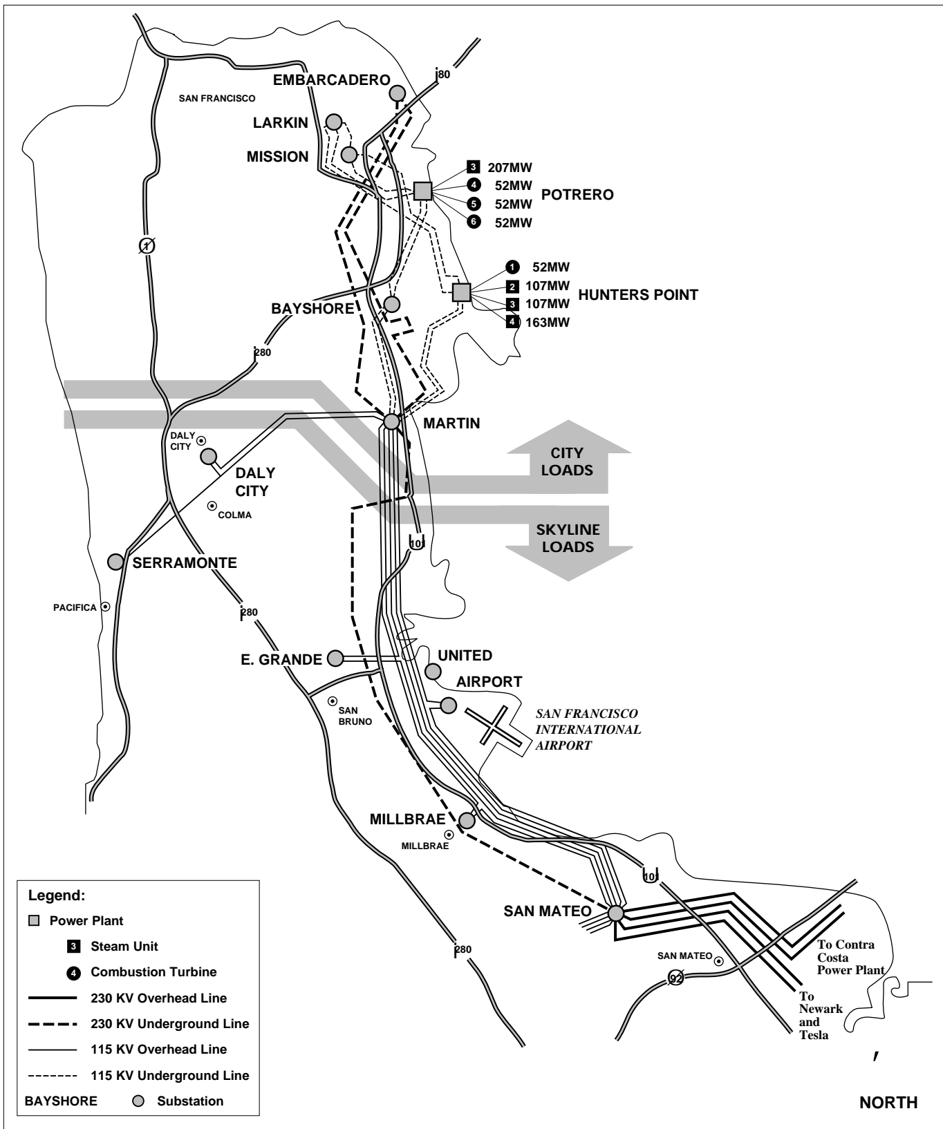
Figure 4.12-1 San Francisco Peninsula Electric Transmission System
