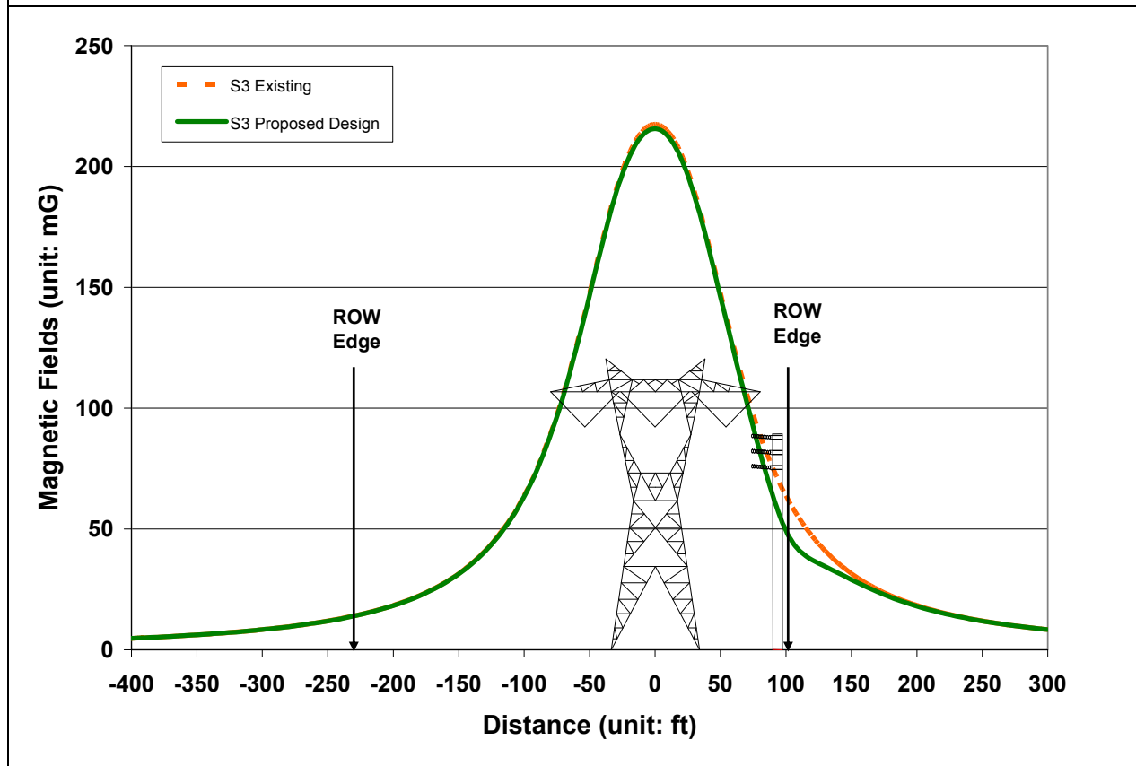
Figure 8. Calculated Magnetic Field Levels 41 for Segment 3 Proposed Etiwanda – Falcon Ridge 66 kV Line and Existing Lugo-Mira Loma No. 3 500 kV T/Ls
