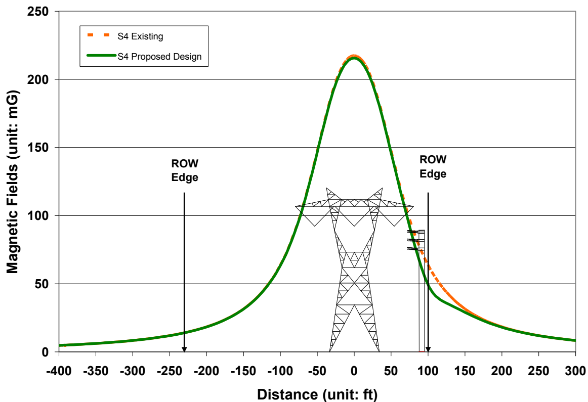
Figure 10. Calculated Magnetic Field Levels 43 for Segment 4 Proposed Etiwanda – Falcon Ridge 66 kV Line and Existing Lugo-Mira Loma No. 3 500 kV T/Ls
