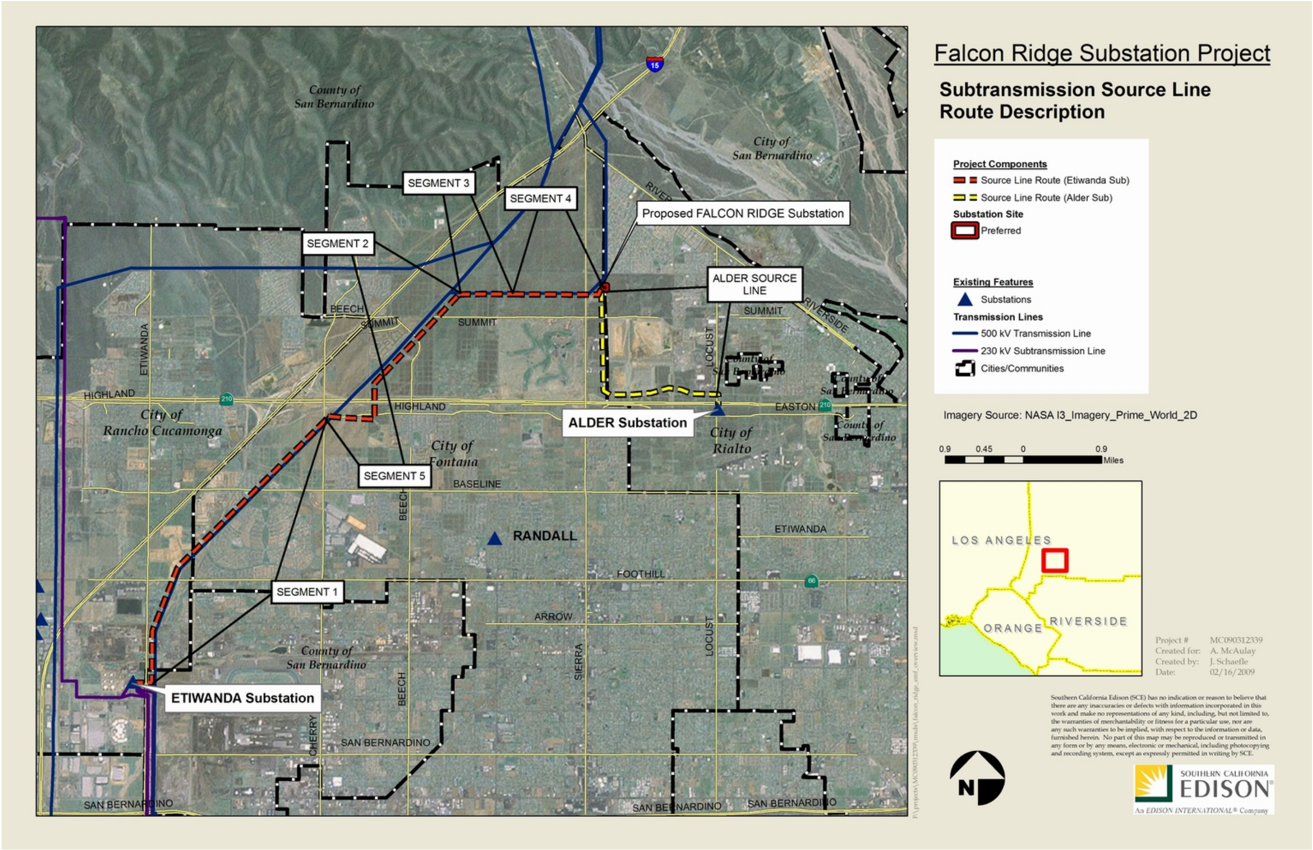
Figure 2. Source Lines Segments for Magnetic Field Analysis
