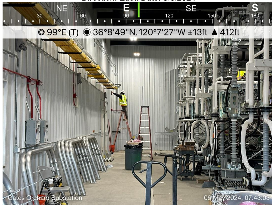
Photo 10. View of hardware installation in enclosure #1. Direction: East. Date: 5/6/2024
