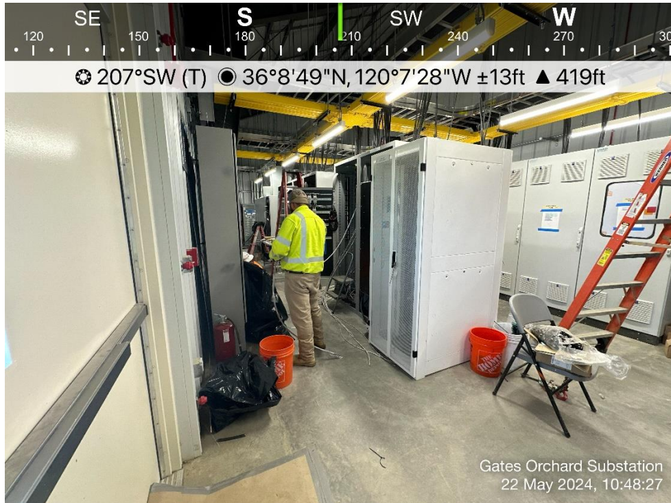
Photo 15. View of crew wiring marshal cabinets in enclosure #1. Direction: Southwest. Date: 5/22/2024
