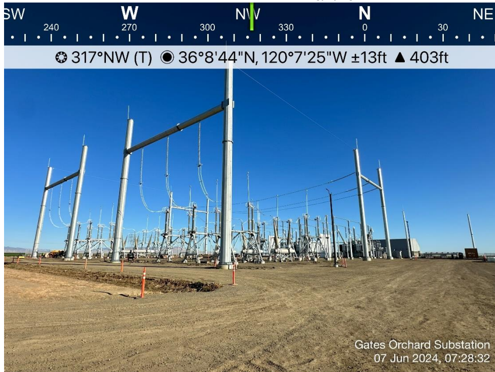
Photo 26. Overview of the Orchard Substation. Direction: Northwest. Date: 6/7/2024
