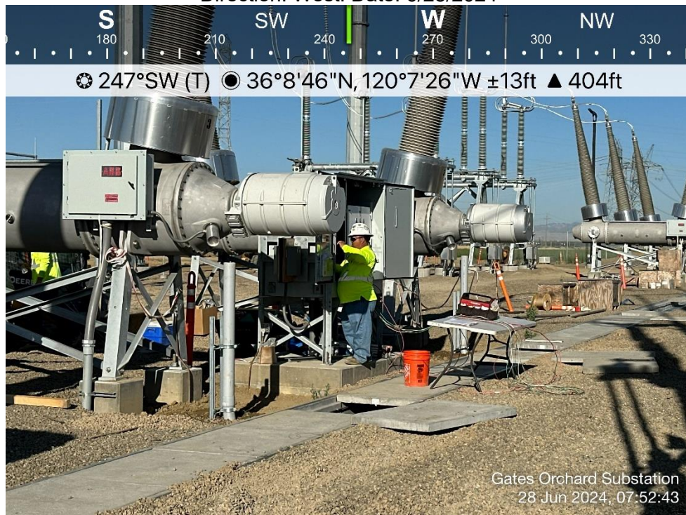
Photo 30. View of crew terminating wires. Direction: West. Date: 6/28/2024
