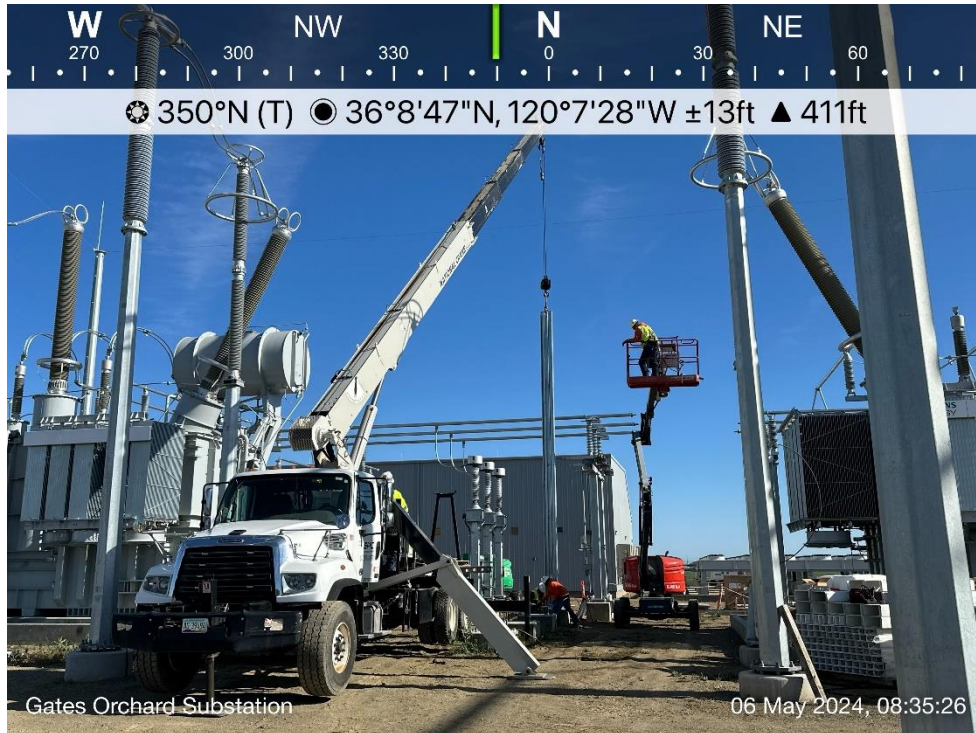
Photo 11. View of fire wall installation. Direction: North. Date: 5/6/2024
