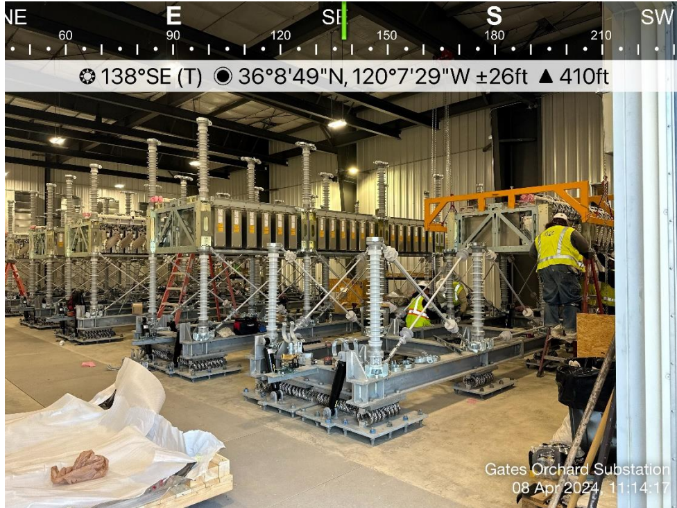
Photo 5. View of crews setting compensators in enclosure #2. Direction: Southeast. Date: 4/8/2024
