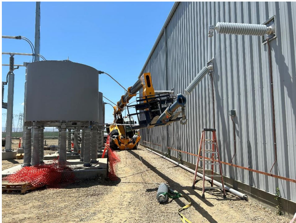
Photo 22. View of reach lift damage of insulator bushing on enclosure #2 that occurred on 6/6/24. Direction: West. Date: 6/7/2024
