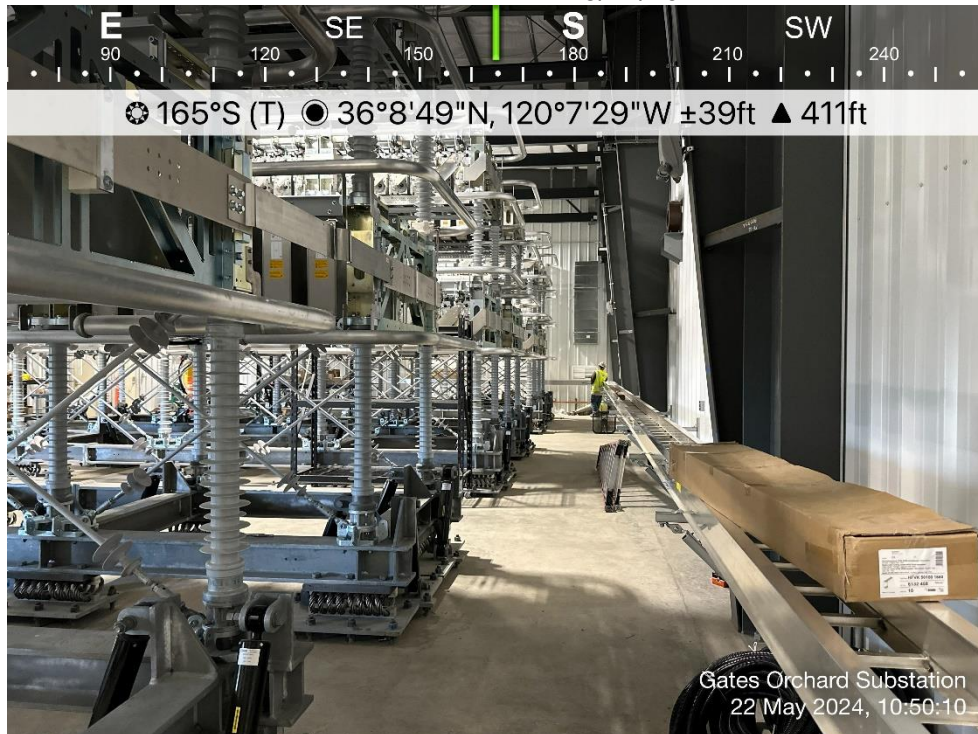
Photo 16. View of crews installing cable trays in enclosure #2. Direction: South. Date: 5/22/2024
