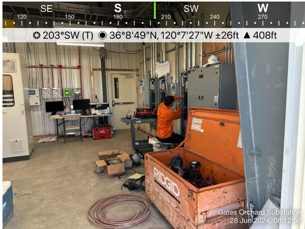
Photo 32. View of crew terminating wires inside enclosure #1. Direction: South. Date: 6/28/2024
