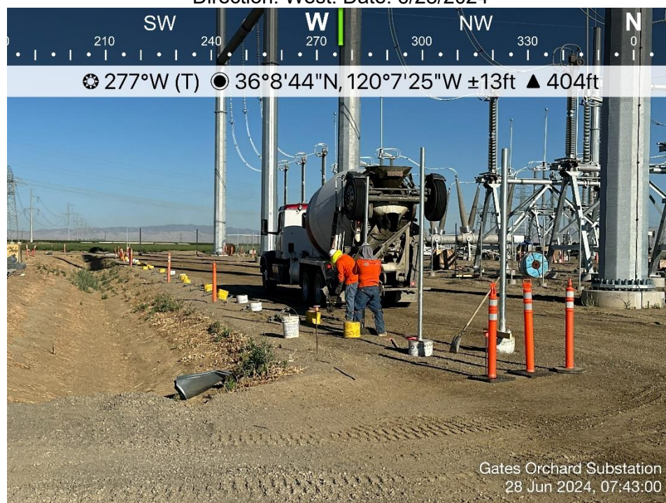
Photo 27. View of fence post installation on the south side of the Orchard Substation. Direction: West. Date: 6/28/2024
