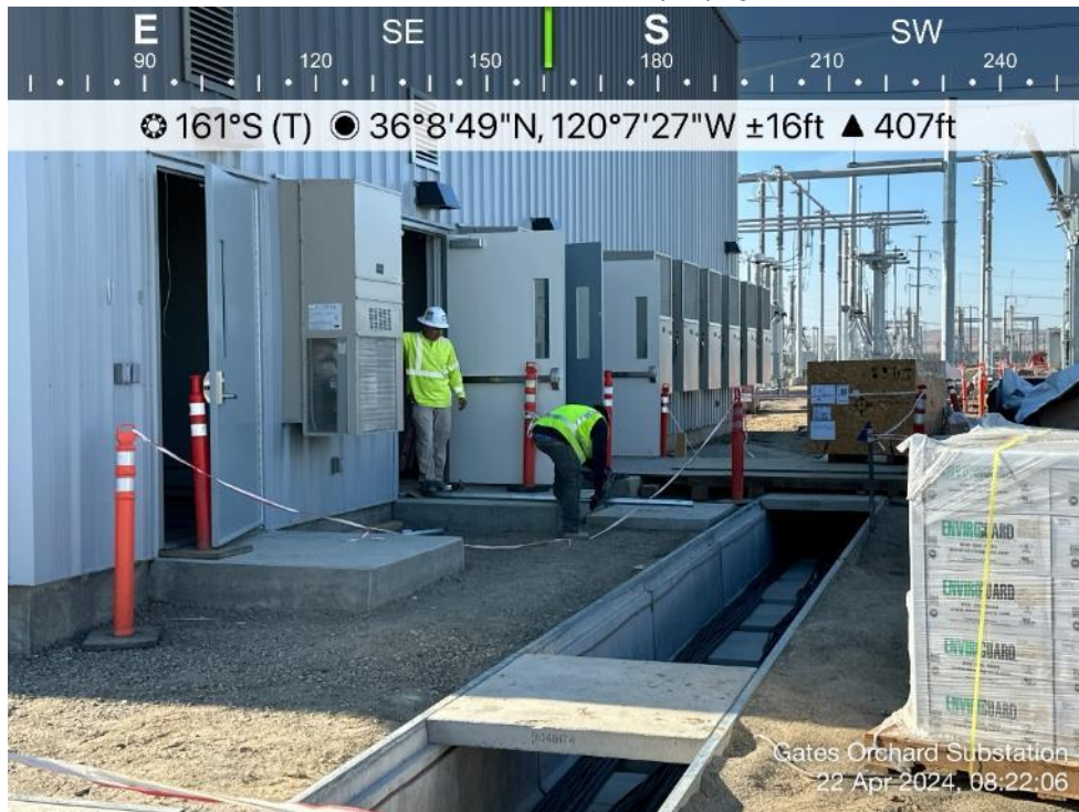
Photo 8. View of panel wiring in enclosure #1. Direction: South. Date: 4/22/2024
