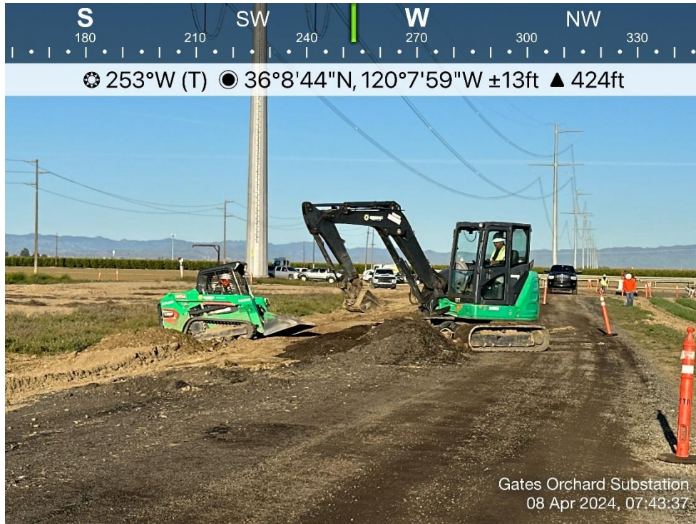
Photo 4. View of structure installation in 97.5kV yard. Direction: West. Date: 4/8/2024
